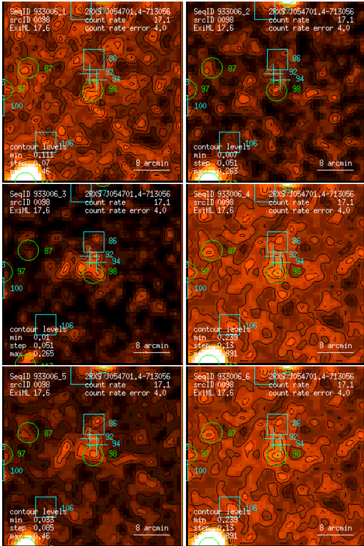
Figure 98: RASS 933006: detection 0098: band rate images, Gaussian filter: (1) PSPC channels 11 – 41, (2) 52 – 90, (3) 91 – 201, (4) 11 – 235, (5) 52 – 201, (6) 11 – 201. Broad band rates in counts/ks. Band rate contour levels in counts/ks/arcmin 2 .
