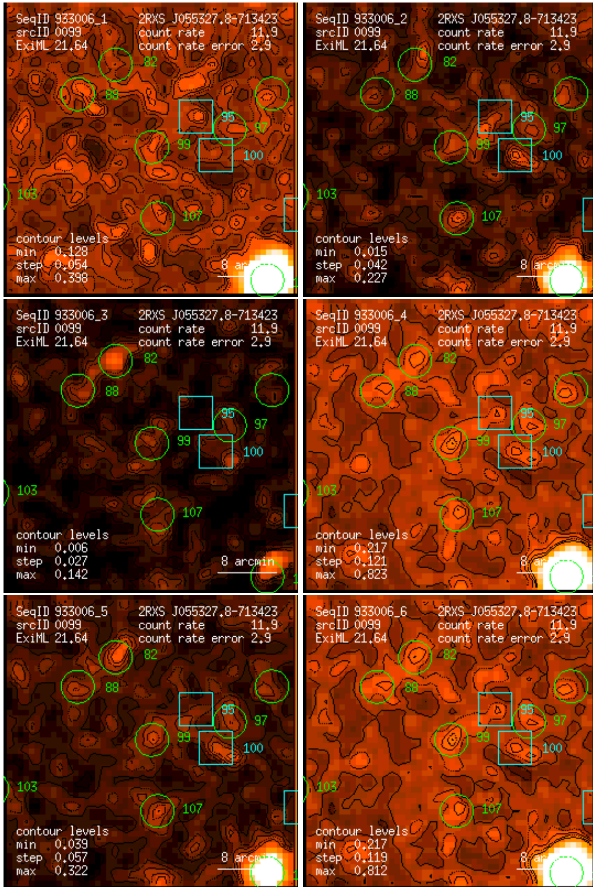
Figure 99: RASS 933006: detection 0099: band rate images, Gaussian filter: (1) PSPC channels 11 – 41, (2) 52 – 90, (3) 91 – 201, (4) 11 – 235, (5) 52 – 201, (6) 11 – 201. Broad band rates in counts/ks. Band rate contour levels in counts/ks/arcmin 2 .
