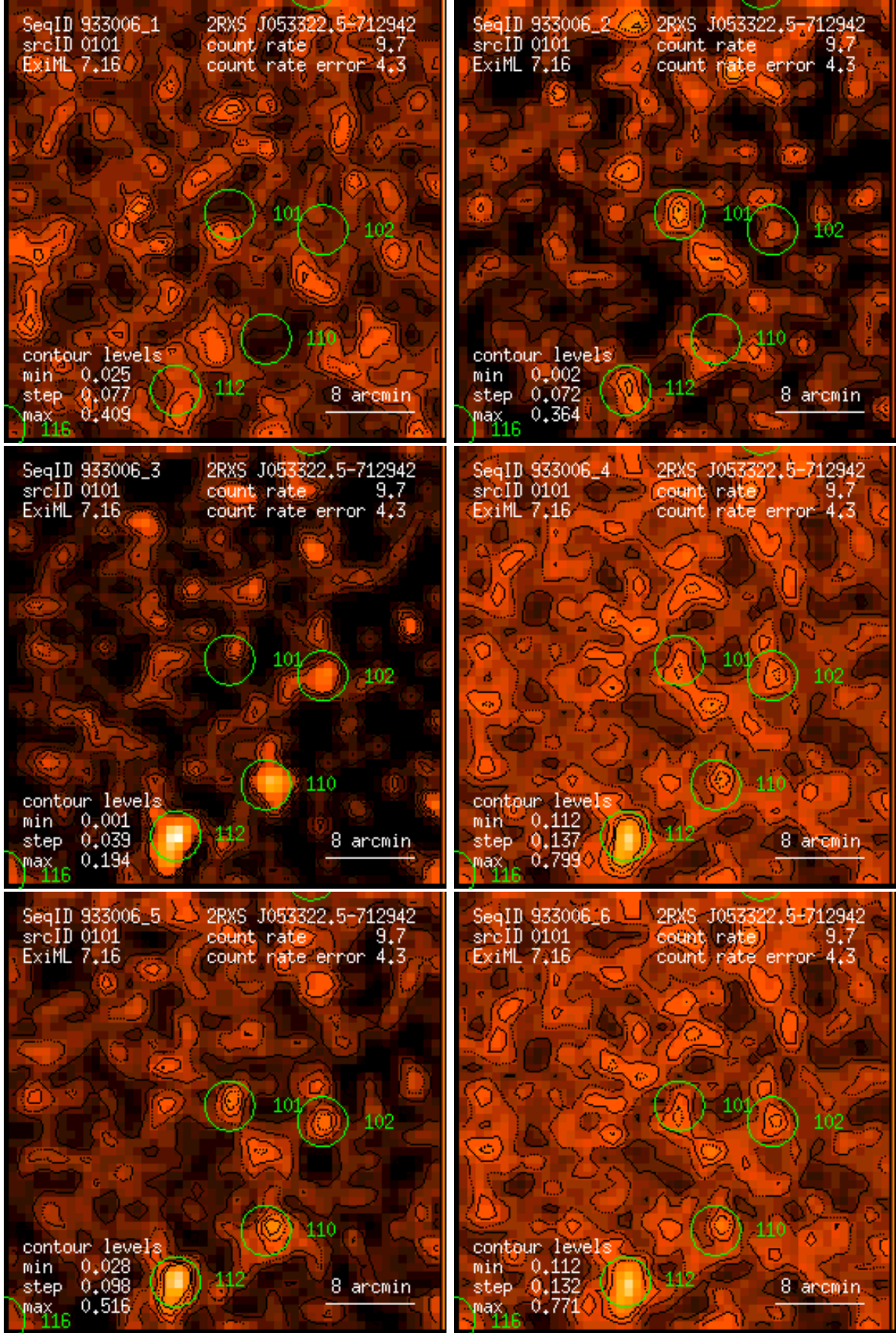
Figure 101: RASS 933006: detection 0101: band rate images, Gaussian filter: (1) PSPC channels 11 – 41, (2) 52 – 90, (3) 91 – 201, (4) 11 – 235, (5) 52 – 201, (6) 11 – 201. Broad band rates in counts/ks. Band rate contour levels in counts/ks/arcmin 2 .
