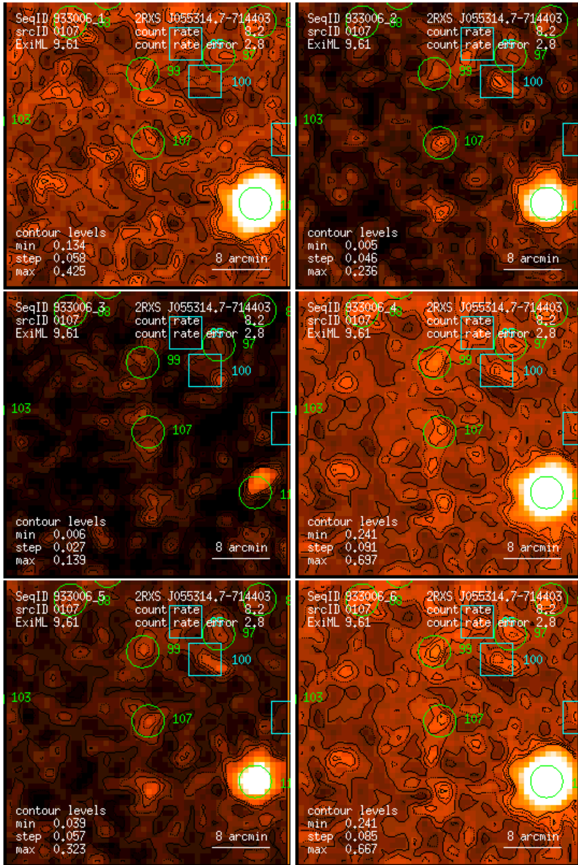
Figure 107: RASS 933006: detection 0107: band rate images, Gaussian filter: (1) PSPC channels 11 – 41, (2) 52 – 90, (3) 91 – 201, (4) 11 – 235, (5) 52 – 201, (6) 11 – 201. Broad band rates in counts/ks. Band rate contour levels in counts/ks/arcmin 2 .
