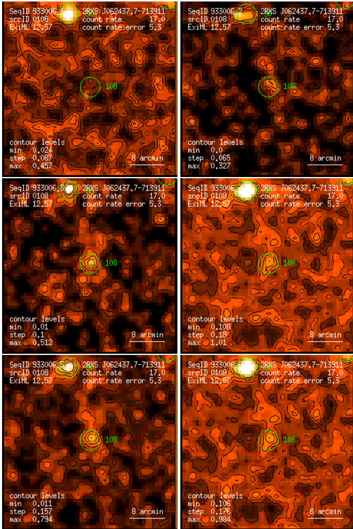
Figure 108: RASS 933006: detection 0108: band rate images, Gaussian filter: (1) PSPC channels 11 – 41, (2) 52 – 90, (3) 91 – 201, (4) 11 – 235, (5) 52 – 201, (6) 11 – 201. Broad band rates in counts/ks. Band rate contour levels in counts/ks/arcmin 2 .
