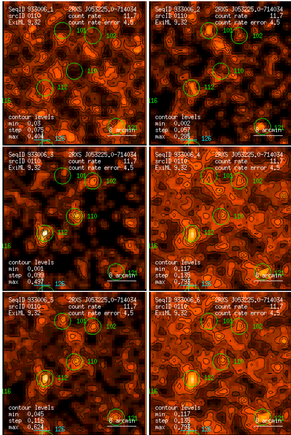
Figure 110: RASS 933006: detection 0110: band rate images, Gaussian filter: (1) PSPC channels 11 – 41, (2) 52 – 90, (3) 91 – 201, (4) 11 – 235, (5) 52 – 201, (6) 11 – 201. Broad band rates in counts/ks. Band rate contour levels in counts/ks/arcmin 2 .
