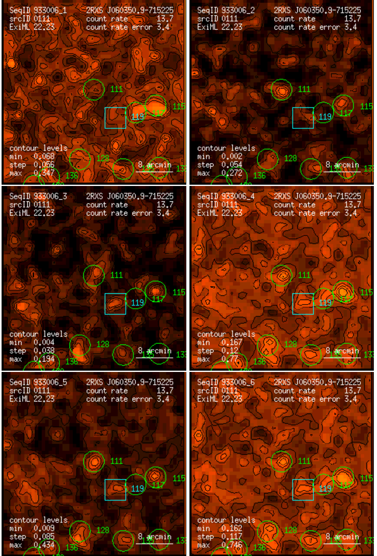
Figure 111: RASS 933006: detection 0111: band rate images, Gaussian filter: (1) PSPC channels 11 – 41, (2) 52 – 90, (3) 91 – 201, (4) 11 – 235, (5) 52 – 201, (6) 11 – 201. Broad band rates in counts/ks. Band rate contour levels in counts/ks/arcmin 2 .
