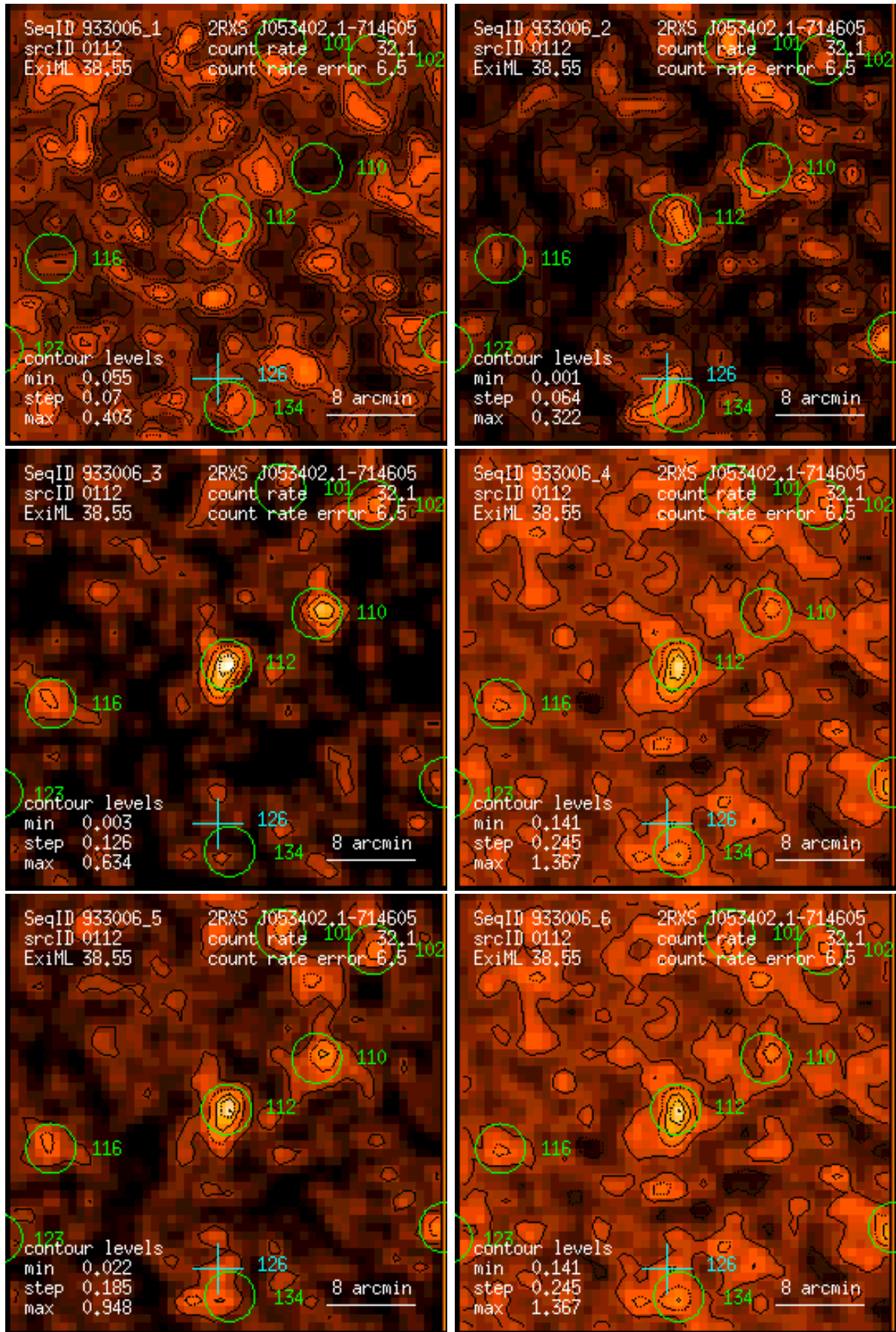
Figure 112: RASS 933006: detection 0112: band rate images, Gaussian filter: (1) PSPC channels 11 – 41, (2) 52 – 90, (3) 91 – 201, (4) 11 – 235, (5) 52 – 201, (6) 11 – 201. Broad band rates in counts/ks. Band rate contour levels in counts/ks/arcmin 2 .
