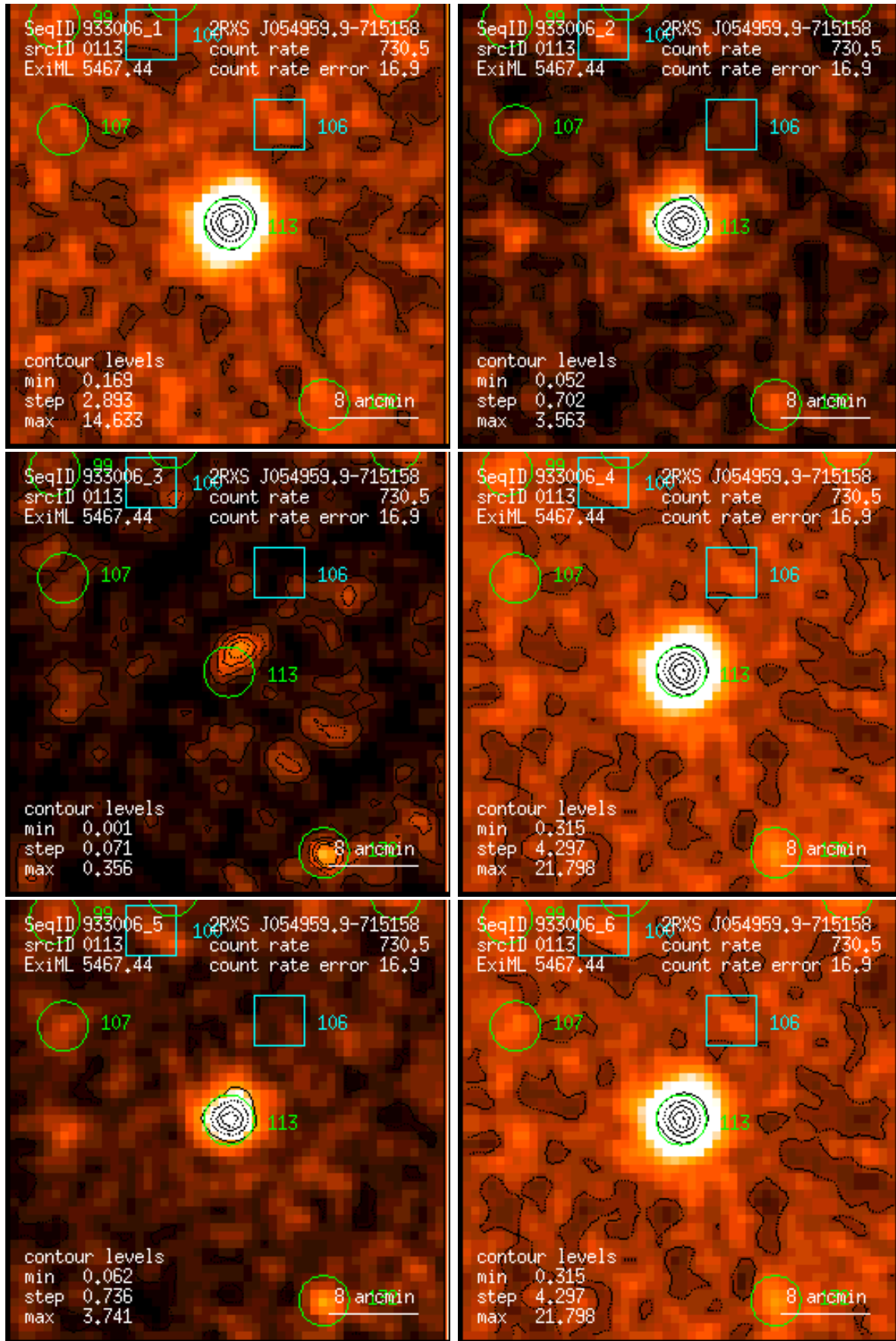
Figure 113: RASS 933006: detection 0113: band rate images, Gaussian filter: (1) PSPC channels 11 – 41, (2) 52 – 90, (3) 91 – 201, (4) 11 – 235, (5) 52 – 201, (6) 11 – 201. Broad band rates in counts/ks. Band rate contour levels in counts/ks/arcmin 2 .
