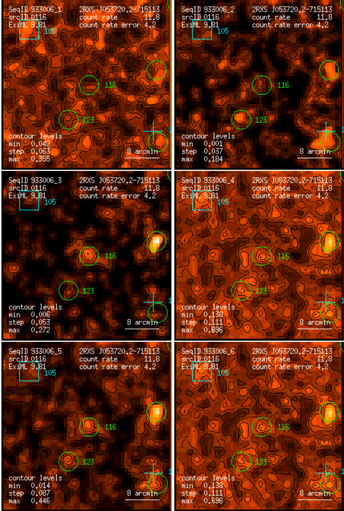
Figure 116: RASS 933006: detection 0116: band rate images, Gaussian filter: (1) PSPC channels 11 – 41, (2) 52 – 90, (3) 91 – 201, (4) 11 – 235, (5) 52 – 201, (6) 11 – 201. Broad band rates in counts/ks. Band rate contour levels in counts/ks/arcmin 2 .
