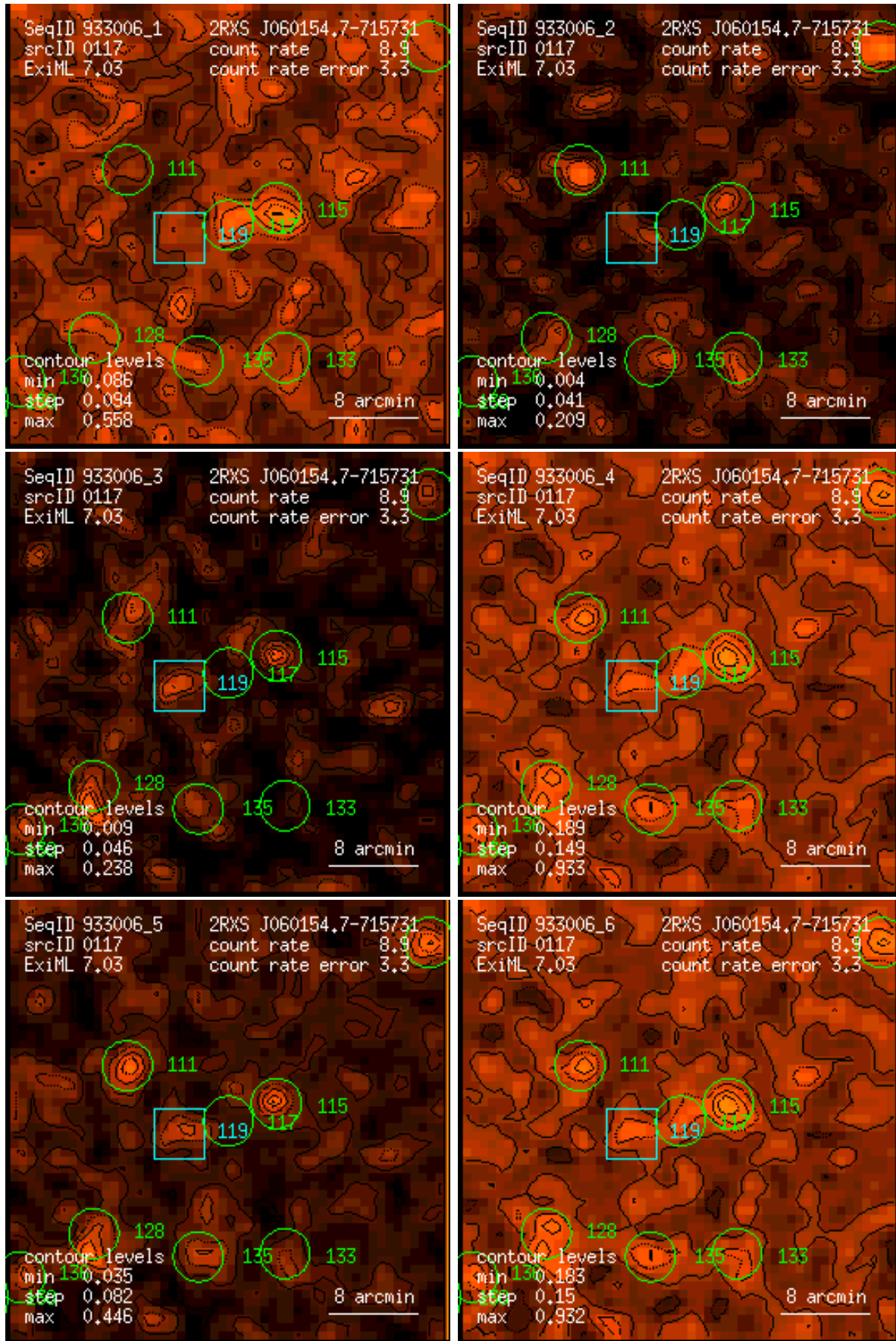
Figure 117: RASS 933006: detection 0117: band rate images, Gaussian filter: (1) PSPC channels 11 – 41, (2) 52 – 90, (3) 91 – 201, (4) 11 – 235, (5) 52 – 201, (6) 11 – 201. Broad band rates in counts/ks. Band rate contour levels in counts/ks/arcmin 2 .
