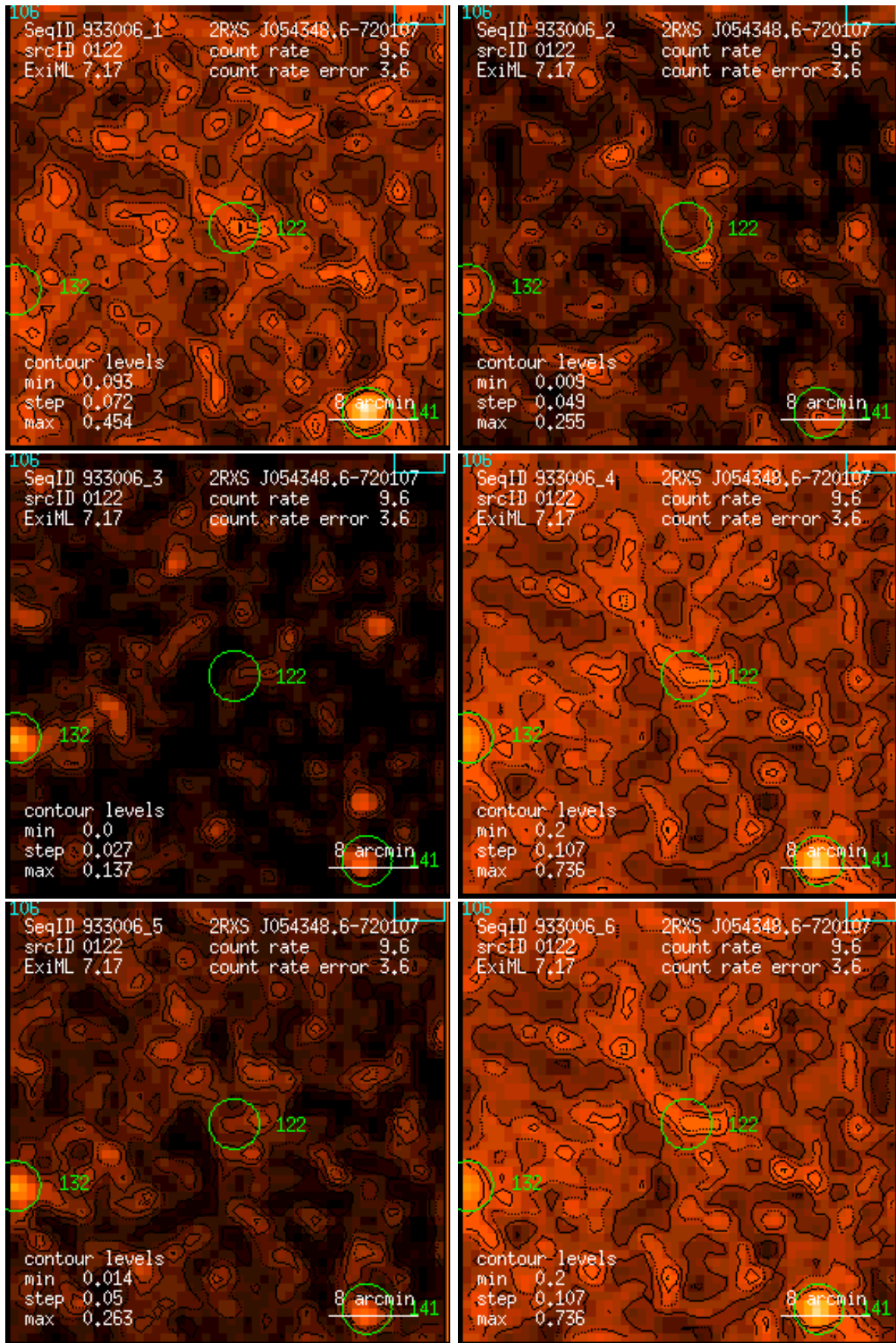
Figure 122: RASS 933006: detection 0122: band rate images, Gaussian filter: (1) PSPC channels 11 – 41, (2) 52 – 90, (3) 91 – 201, (4) 11 – 235, (5) 52 – 201, (6) 11 – 201. Broad band rates in counts/ks. Band rate contour levels in counts/ks/arcmin 2 .
