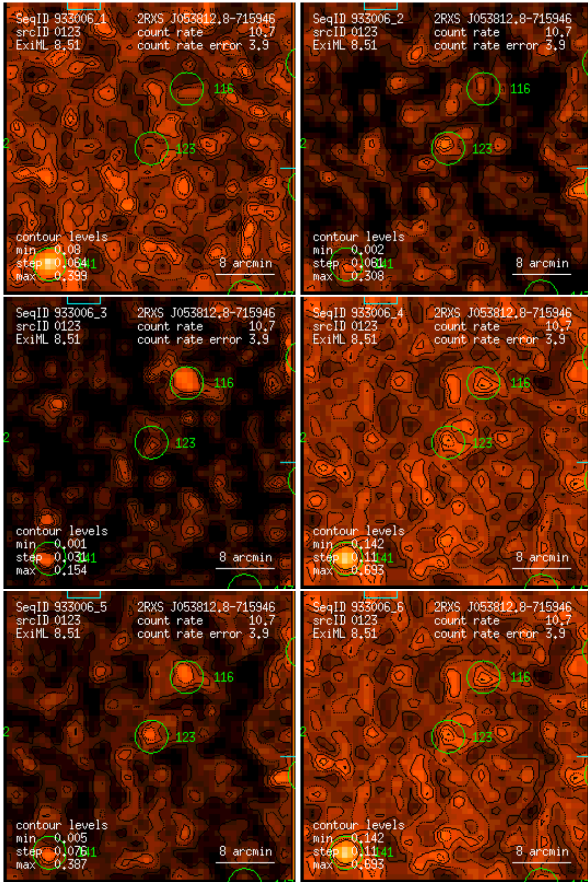
Figure 123: RASS 933006: detection 0123: band rate images, Gaussian filter: (1) PSPC channels 11 – 41, (2) 52 – 90, (3) 91 – 201, (4) 11 – 235, (5) 52 – 201, (6) 11 – 201. Broad band rates in counts/ks. Band rate contour levels in counts/ks/arcmin 2 .
