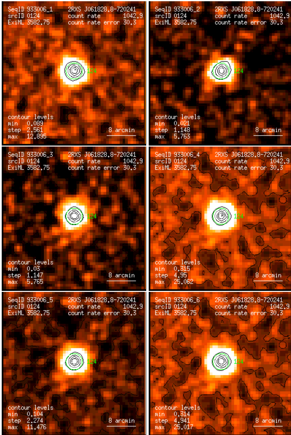
Figure 124: RASS 933006: detection 0124: band rate images, Gaussian filter: (1) PSPC channels 11 – 41, (2) 52 – 90, (3) 91 – 201, (4) 11 – 235, (5) 52 – 201, (6) 11 – 201. Broad band rates in counts/ks. Band rate contour levels in counts/ks/arcmin 2 .
