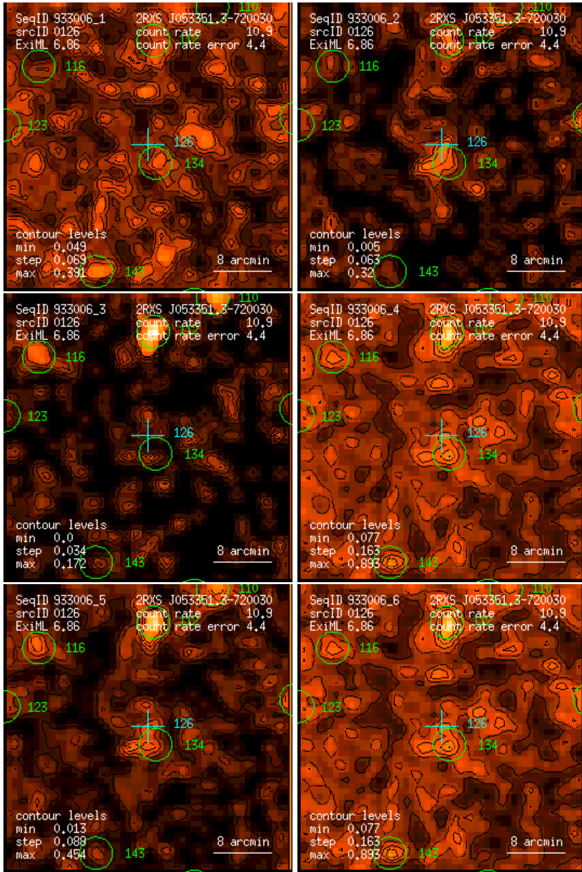
Figure 126: RASS 933006: detection 0126: band rate images, Gaussian filter: (1) PSPC channels 11 – 41, (2) 52 – 90, (3) 91 – 201, (4) 11 – 235, (5) 52 – 201, (6) 11 – 201. Broad band rates in counts/ks. Band rate contour levels in counts/ks/arcmin 2 .
