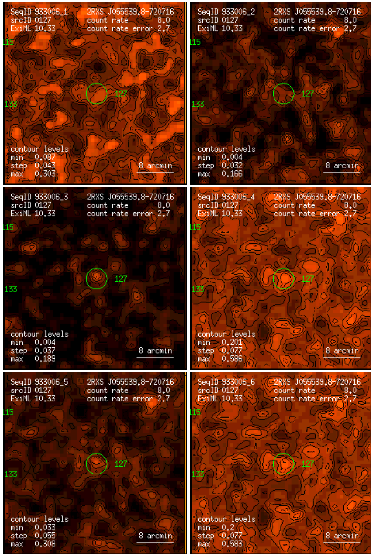
Figure 127: RASS 933006: detection 0127: band rate images, Gaussian filter: (1) PSPC channels 11 – 41, (2) 52 – 90, (3) 91 – 201, (4) 11 – 235, (5) 52 – 201, (6) 11 – 201. Broad band rates in counts/ks. Band rate contour levels in counts/ks/arcmin 2 .
