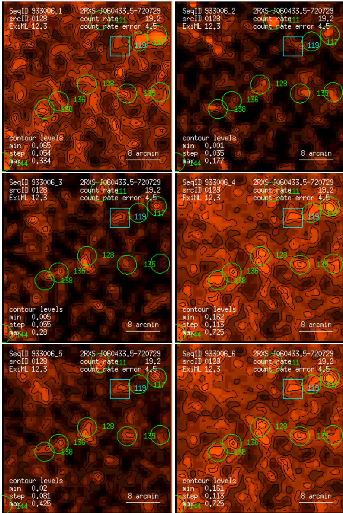
Figure 128: RASS 933006: detection 0128: band rate images, Gaussian filter: (1) PSPC channels 11 – 41, (2) 52 – 90, (3) 91 – 201, (4) 11 – 235, (5) 52 – 201, (6) 11 – 201. Broad band rates in counts/ks. Band rate contour levels in counts/ks/arcmin 2 .
