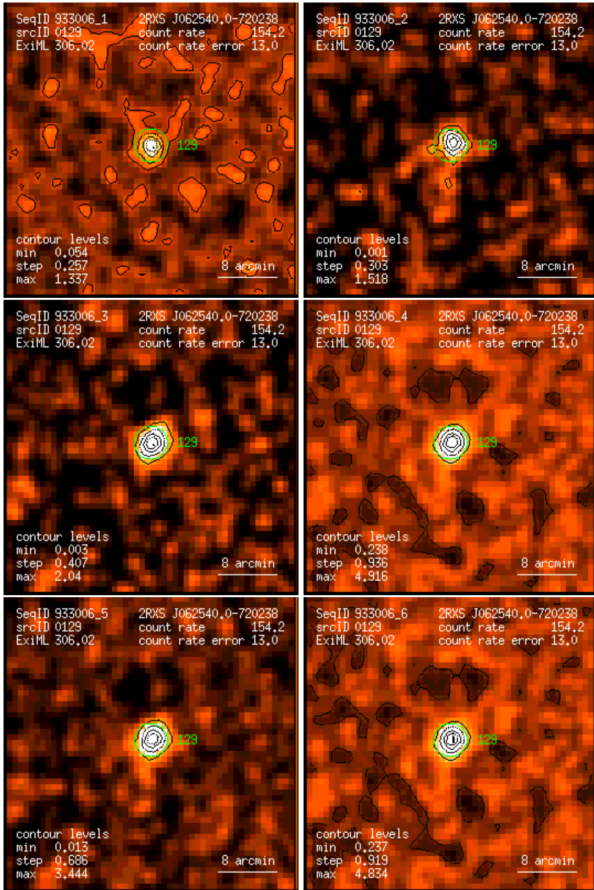
Figure 129: RASS 933006: detection 0129: band rate images, Gaussian filter: (1) PSPC channels 11 – 41, (2) 52 – 90, (3) 91 – 201, (4) 11 – 235, (5) 52 – 201, (6) 11 – 201. Broad band rates in counts/ks. Band rate contour levels in counts/ks/arcmin 2 .
