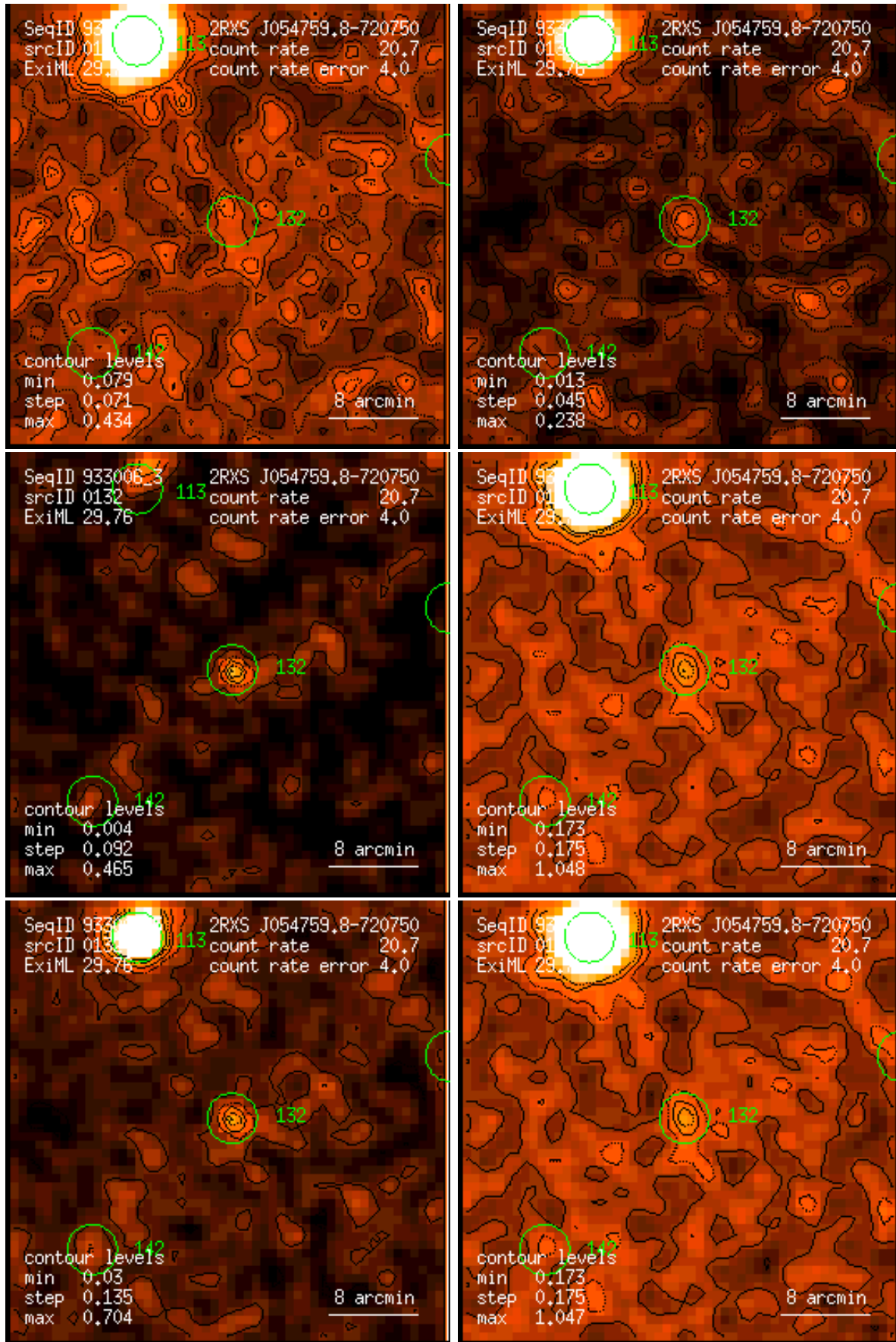
Figure 132: RASS 933006: detection 0132: band rate images, Gaussian filter: (1) PSPC channels 11 – 41, (2) 52 – 90, (3) 91 – 201, (4) 11 – 235, (5) 52 – 201, (6) 11 – 201. Broad band rates in counts/ks. Band rate contour levels in counts/ks/arcmin 2 .
