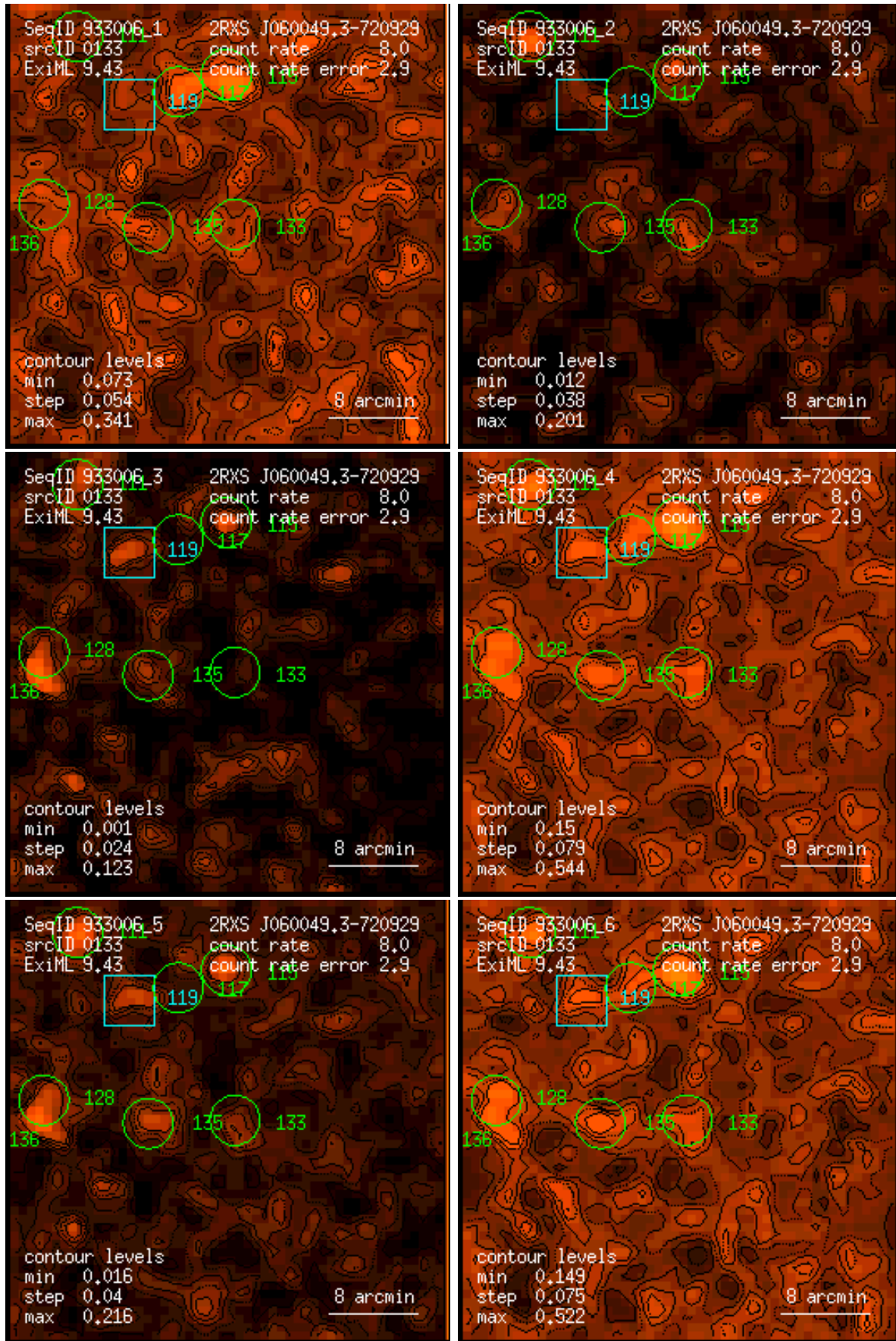
Figure 133: RASS 933006: detection 0133: band rate images, Gaussian filter: (1) PSPC channels 11 – 41, (2) 52 – 90, (3) 91 – 201, (4) 11 – 235, (5) 52 – 201, (6) 11 – 201. Broad band rates in counts/ks. Band rate contour levels in counts/ks/arcmin 2 .
