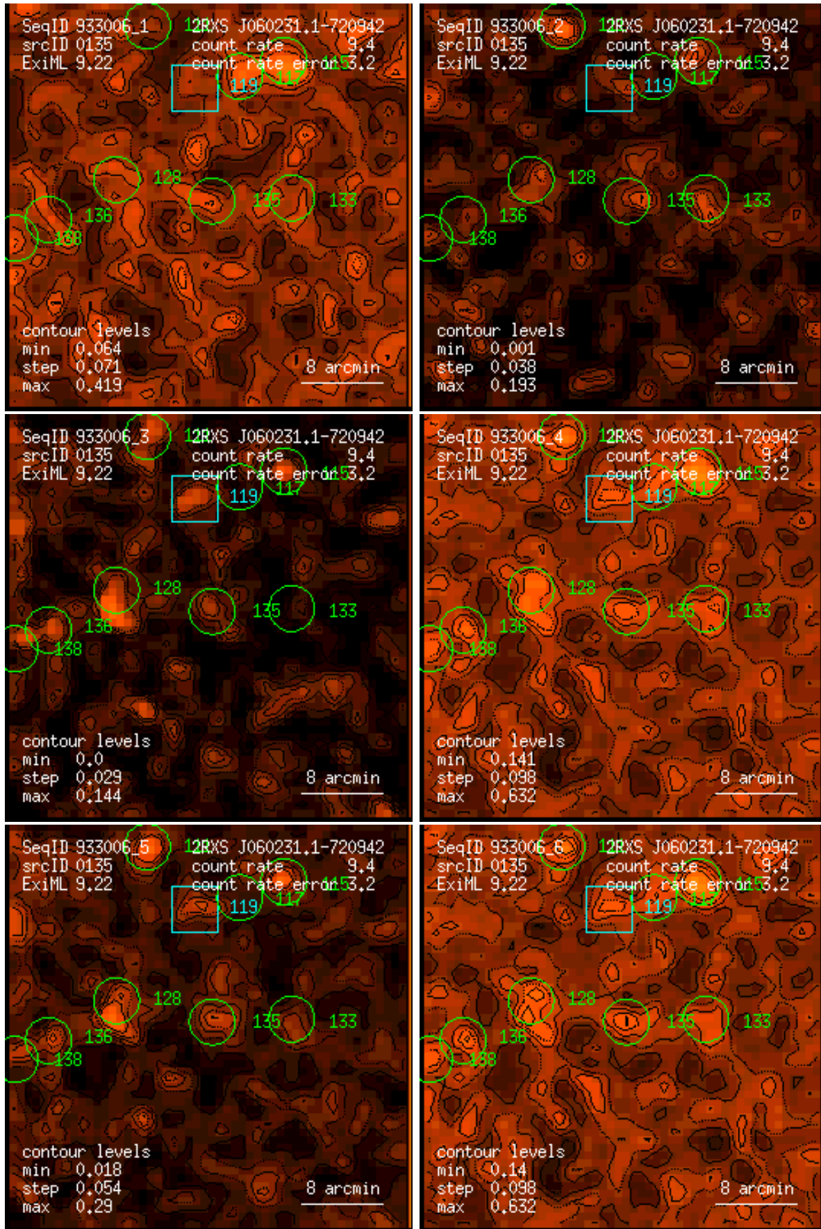
Figure 135: RASS 933006: detection 0135: band rate images, Gaussian filter: (1) PSPC channels 11 – 41, (2) 52 – 90, (3) 91 – 201, (4) 11 – 235, (5) 52 – 201, (6) 11 – 201. Broad band rates in counts/ks. Band rate contour levels in counts/ks/arcmin 2 .
