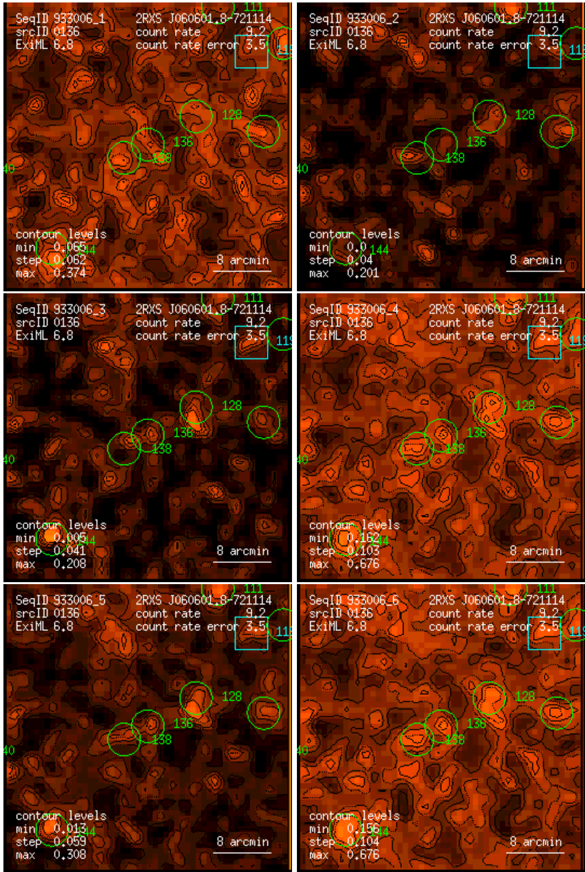
Figure 136: RASS 933006: detection 0136: band rate images, Gaussian filter: (1) PSPC channels 11 – 41, (2) 52 – 90, (3) 91 – 201, (4) 11 – 235, (5) 52 – 201, (6) 11 – 201. Broad band rates in counts/ks. Band rate contour levels in counts/ks/arcmin 2 .
