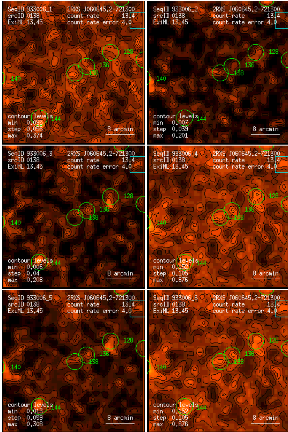
Figure 138: RASS 933006: detection 0138: band rate images, Gaussian filter: (1) PSPC channels 11 – 41, (2) 52 – 90, (3) 91 – 201, (4) 11 – 235, (5) 52 – 201, (6) 11 – 201. Broad band rates in counts/ks. Band rate contour levels in counts/ks/arcmin 2 .
