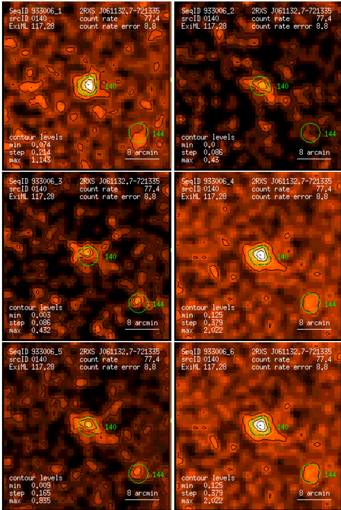
Figure 140: RASS 933006: detection 0140: band rate images, Gaussian filter: (1) PSPC channels 11 – 41, (2) 52 – 90, (3) 91 – 201, (4) 11 – 235, (5) 52 – 201, (6) 11 – 201. Broad band rates in counts/ks. Band rate contour levels in counts/ks/arcmin 2 .
