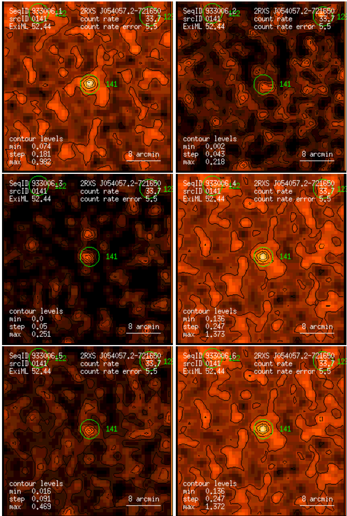
Figure 141: RASS 933006: detection 0141: band rate images, Gaussian filter: (1) PSPC channels 11 – 41, (2) 52 – 90, (3) 91 – 201, (4) 11 – 235, (5) 52 – 201, (6) 11 – 201. Broad band rates in counts/ks. Band rate contour levels in counts/ks/arcmin 2 .
