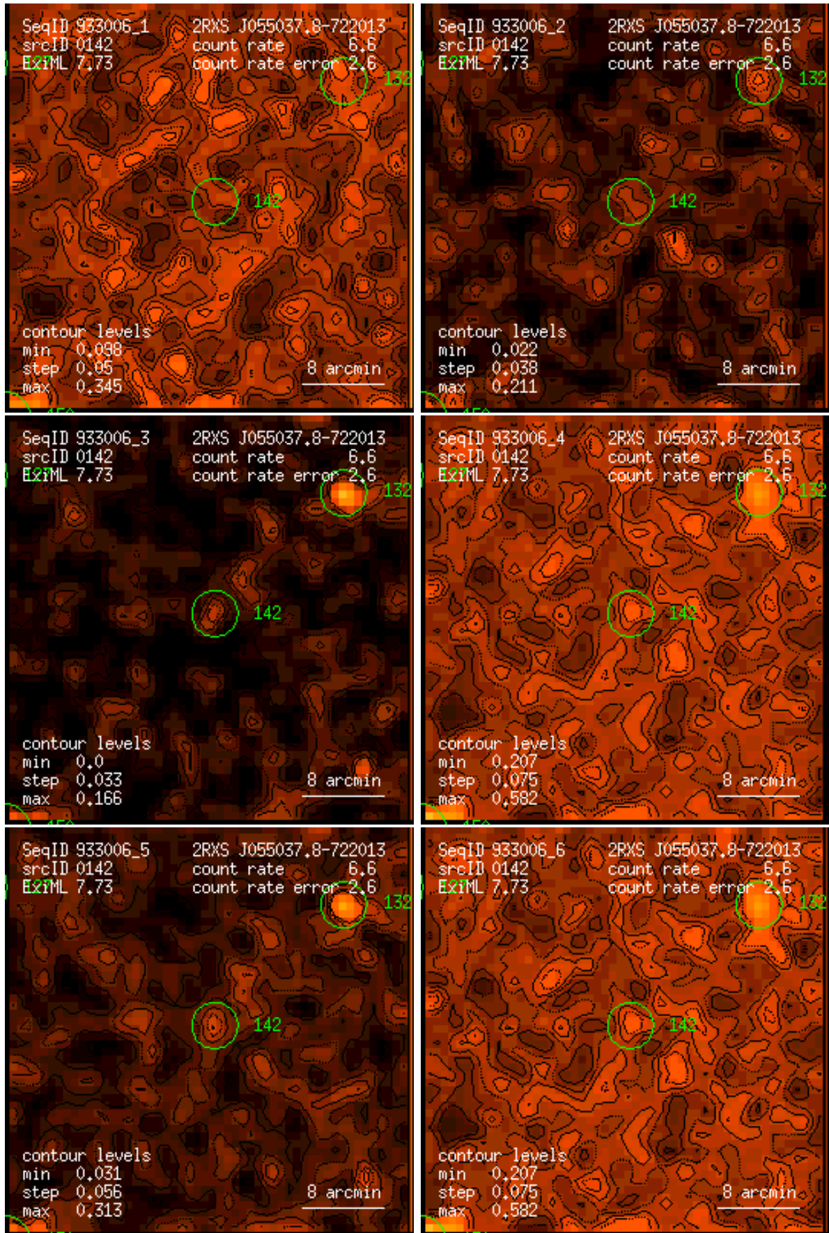
Figure 142: RASS 933006: detection 0142: band rate images, Gaussian filter: (1) PSPC channels 11 – 41, (2) 52 – 90, (3) 91 – 201, (4) 11 – 235, (5) 52 – 201, (6) 11 – 201. Broad band rates in counts/ks. Band rate contour levels in counts/ks/arcmin 2 .
