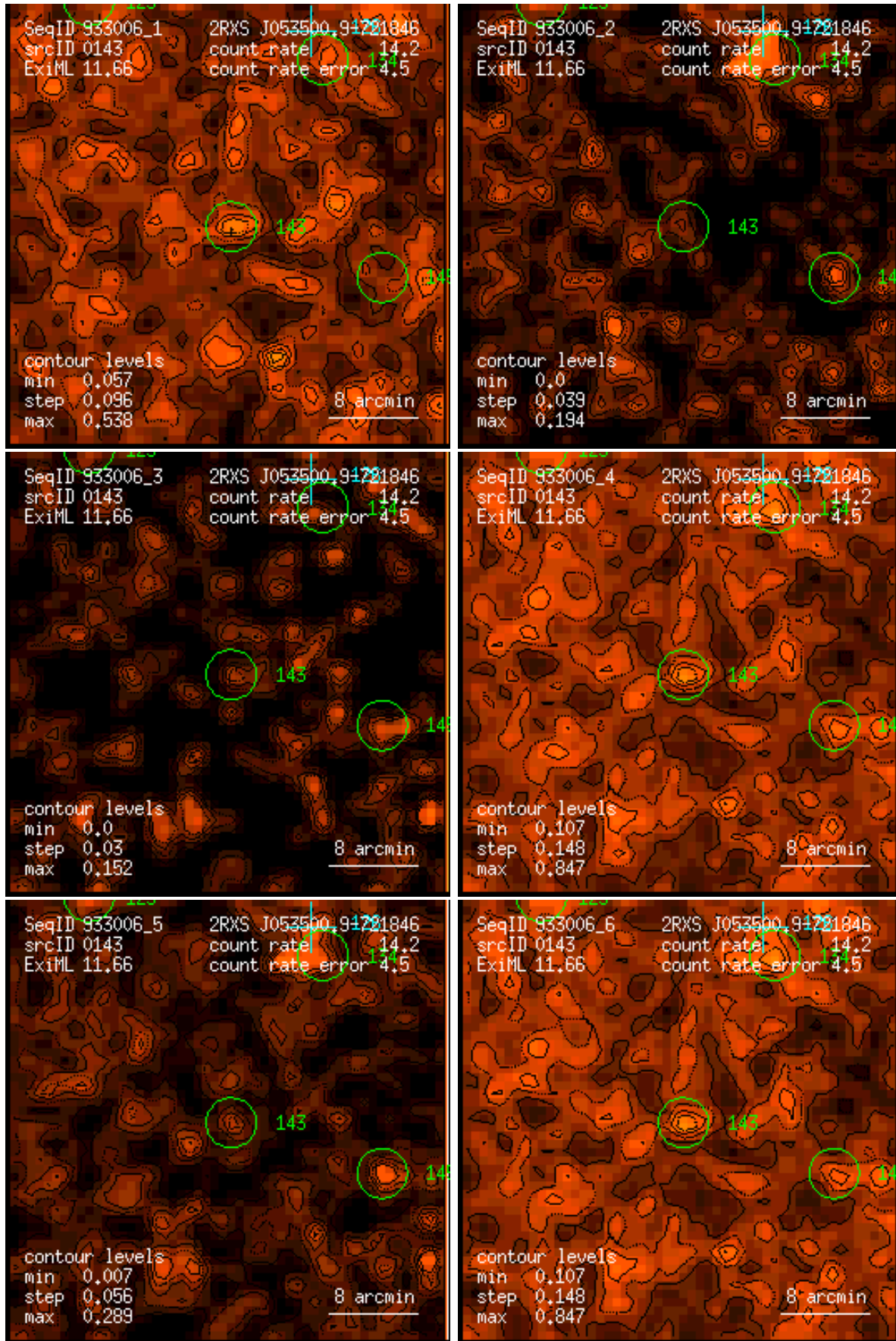
Figure 143: RASS 933006: detection 0143: band rate images, Gaussian filter: (1) PSPC channels 11 – 41, (2) 52 – 90, (3) 91 – 201, (4) 11 – 235, (5) 52 – 201, (6) 11 – 201. Broad band rates in counts/ks. Band rate contour levels in counts/ks/arcmin 2 .
