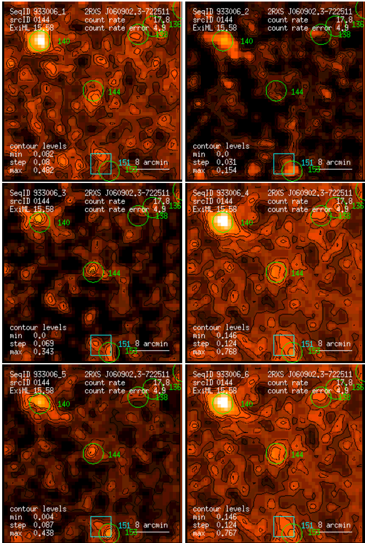
Figure 144: RASS 933006: detection 0144: band rate images, Gaussian filter: (1) PSPC channels 11 – 41, (2) 52 – 90, (3) 91 – 201, (4) 11 – 235, (5) 52 – 201, (6) 11 – 201. Broad band rates in counts/ks. Band rate contour levels in counts/ks/arcmin 2 .
