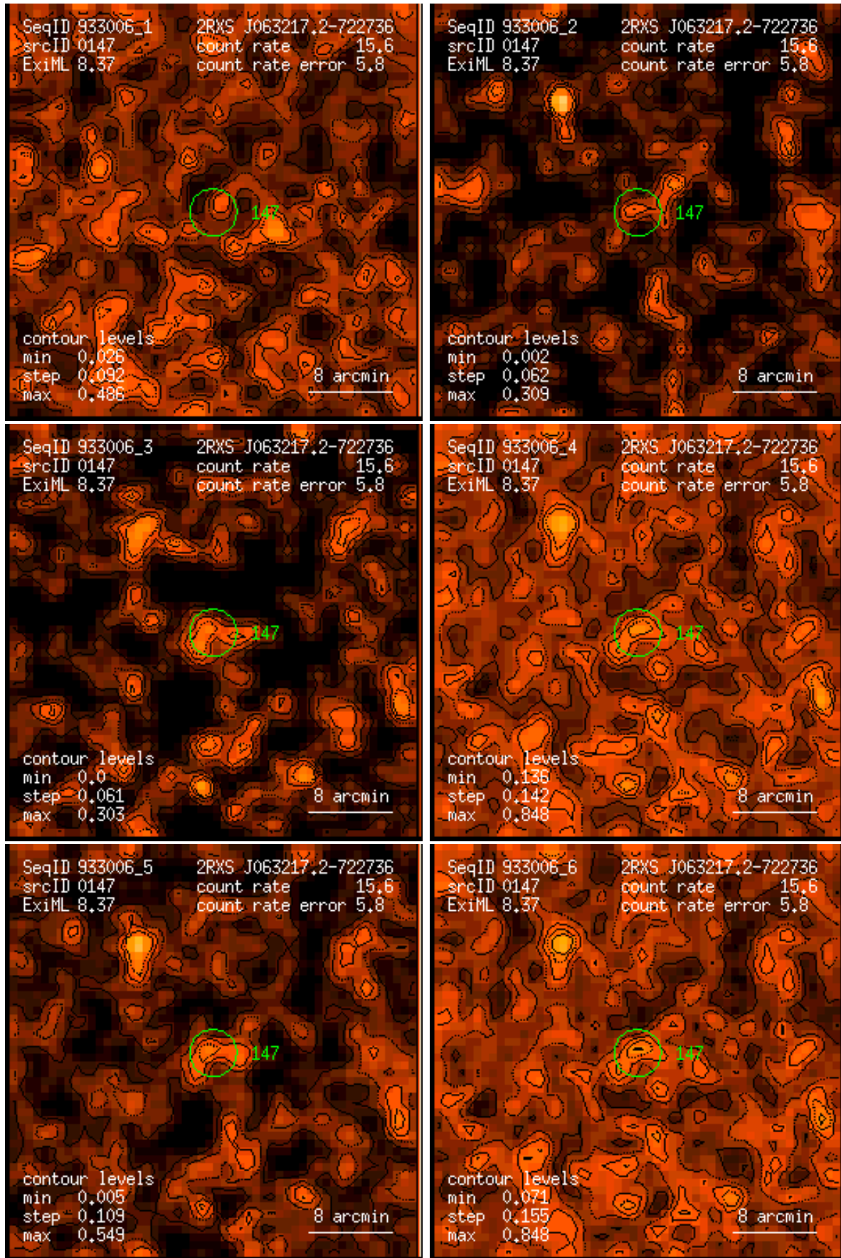
Figure 147: RASS 933006: detection 0147: band rate images, Gaussian filter: (1) PSPC channels 11 – 41, (2) 52 – 90, (3) 91 – 201, (4) 11 – 235, (5) 52 – 201, (6) 11 – 201. Broad band rates in counts/ks. Band rate contour levels in counts/ks/arcmin 2 .
