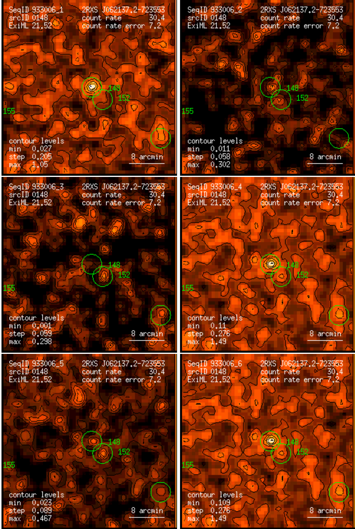
Figure 148: RASS 933006: detection 0148: band rate images, Gaussian filter: (1) PSPC channels 11 – 41, (2) 52 – 90, (3) 91 – 201, (4) 11 – 235, (5) 52 – 201, (6) 11 – 201. Broad band rates in counts/ks. Band rate contour levels in counts/ks/arcmin 2 .
