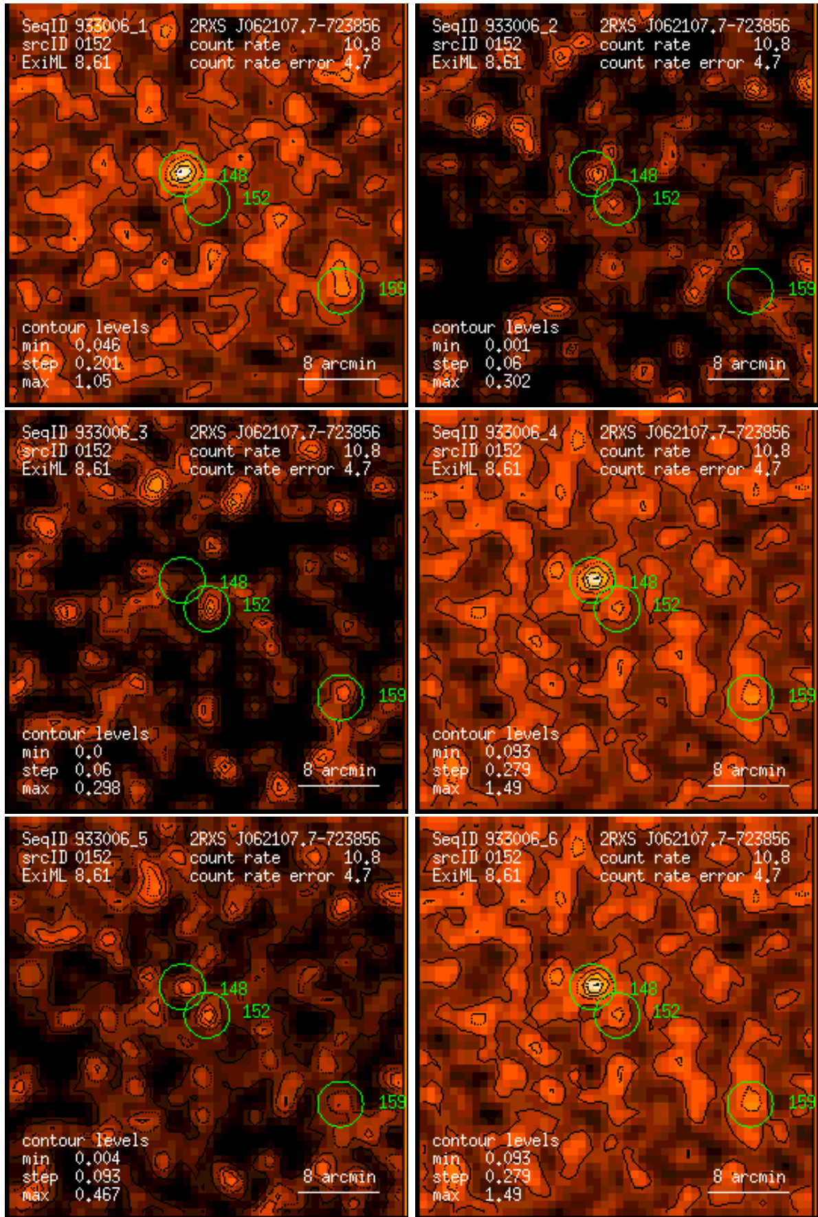
Figure 152: RASS 933006: detection 0152: band rate images, Gaussian filter: (1) PSPC channels 11 – 41, (2) 52 – 90, (3) 91 – 201, (4) 11 – 235, (5) 52 – 201, (6) 11 – 201. Broad band rates in counts/ks. Band rate contour levels in counts/ks/arcmin 2 .
