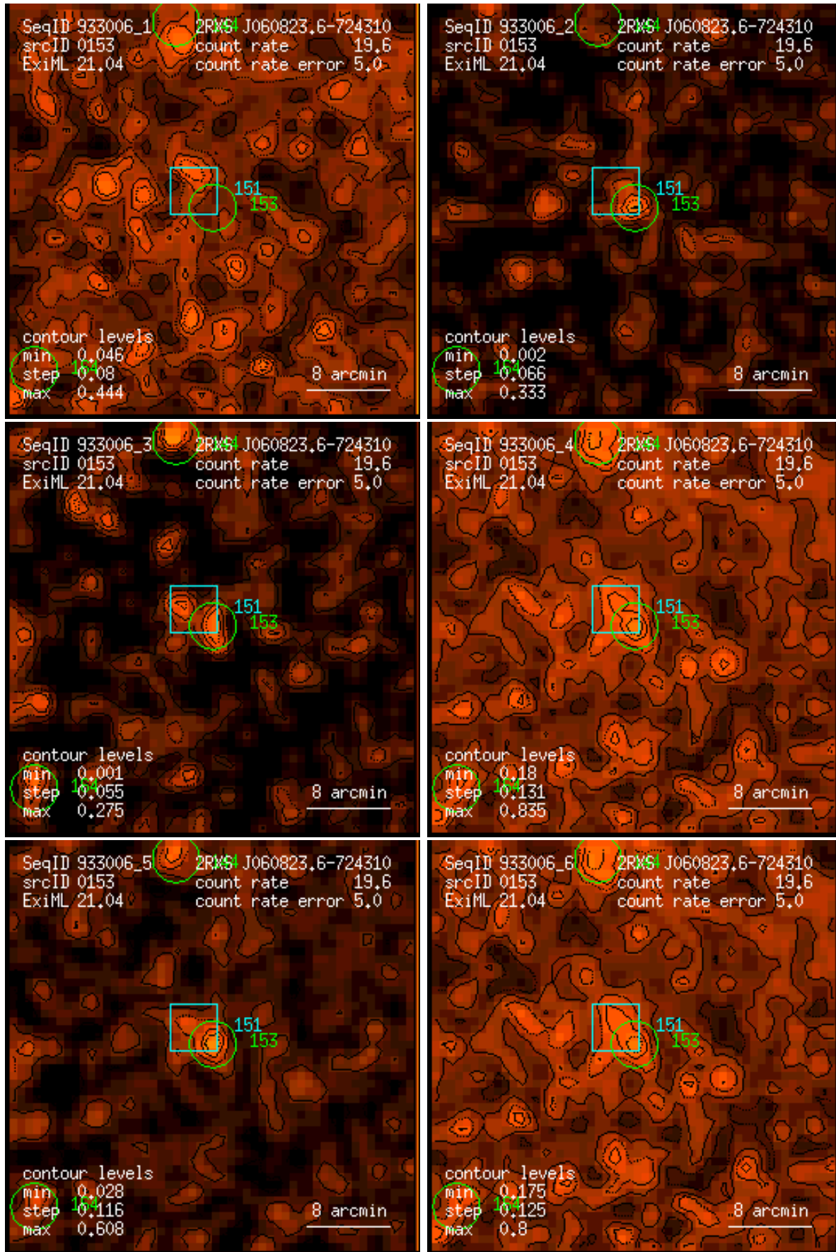
Figure 153: RASS 933006: detection 0153: band rate images, Gaussian filter: (1) PSPC channels 11 – 41, (2) 52 – 90, (3) 91 – 201, (4) 11 – 235, (5) 52 – 201, (6) 11 – 201. Broad band rates in counts/ks. Band rate contour levels in counts/ks/arcmin 2 .
