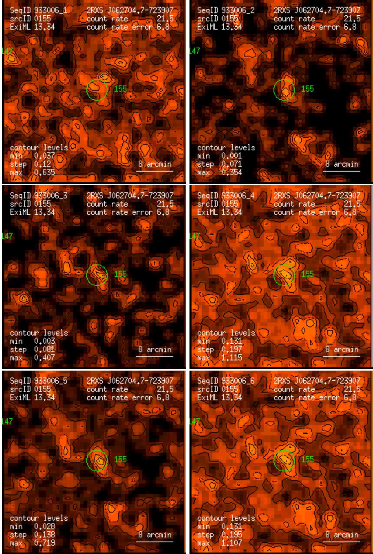
Figure 155: RASS 933006: detection 0155: band rate images, Gaussian filter: (1) PSPC channels 11 – 41, (2) 52 – 90, (3) 91 – 201, (4) 11 – 235, (5) 52 – 201, (6) 11 – 201. Broad band rates in counts/ks. Band rate contour levels in counts/ks/arcmin 2 .
