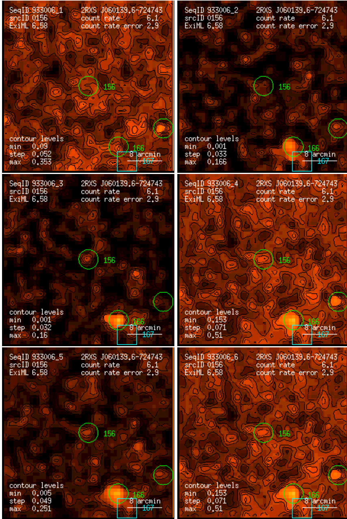
Figure 156: RASS 933006: detection 0156: band rate images, Gaussian filter: (1) PSPC channels 11 – 41, (2) 52 – 90, (3) 91 – 201, (4) 11 – 235, (5) 52 – 201, (6) 11 – 201. Broad band rates in counts/ks. Band rate contour levels in counts/ks/arcmin 2 .
