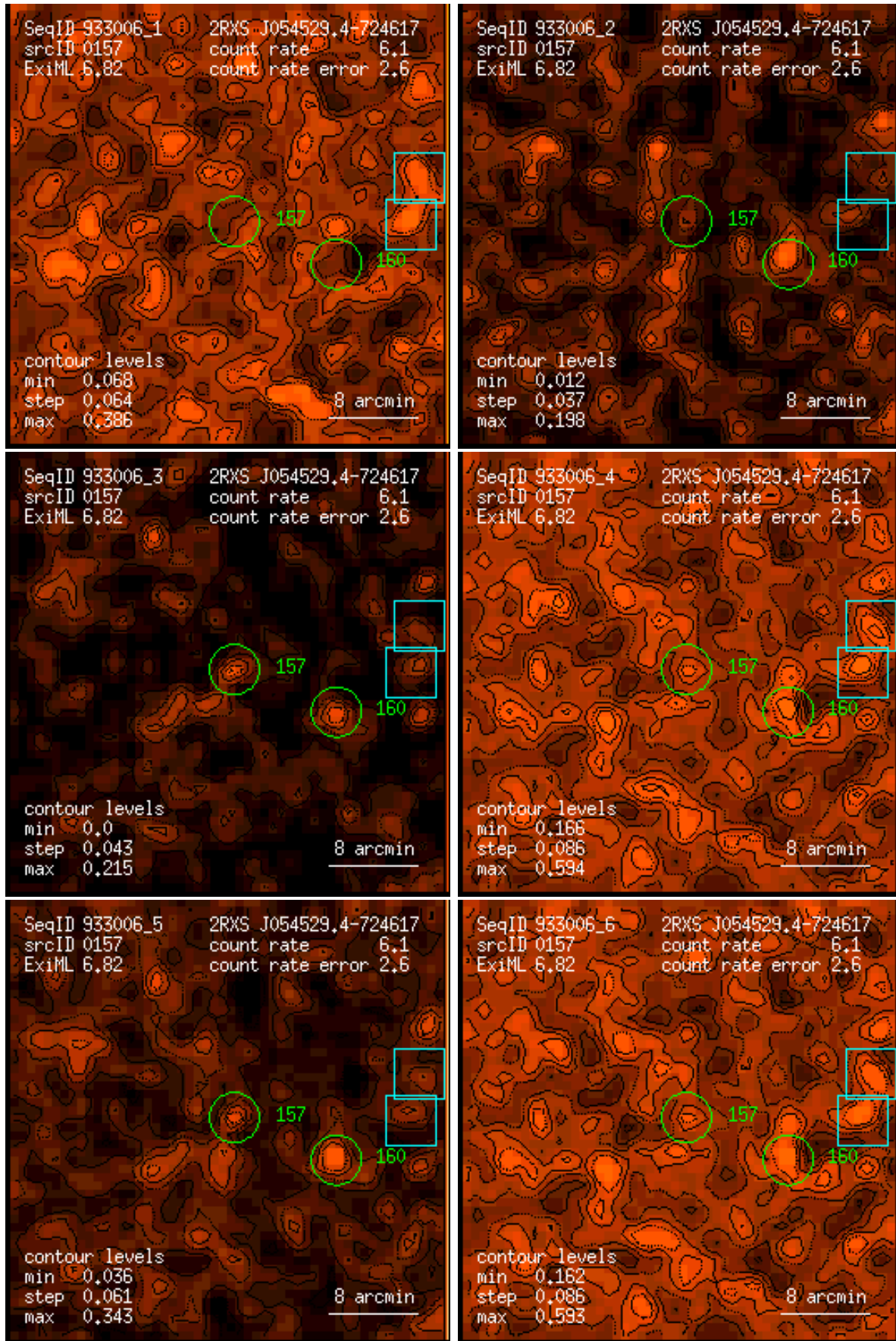
Figure 157: RASS 933006: detection 0157: band rate images, Gaussian filter: (1) PSPC channels 11 – 41, (2) 52 – 90, (3) 91 – 201, (4) 11 – 235, (5) 52 – 201, (6) 11 – 201. Broad band rates in counts/ks. Band rate contour levels in counts/ks/arcmin 2 .
