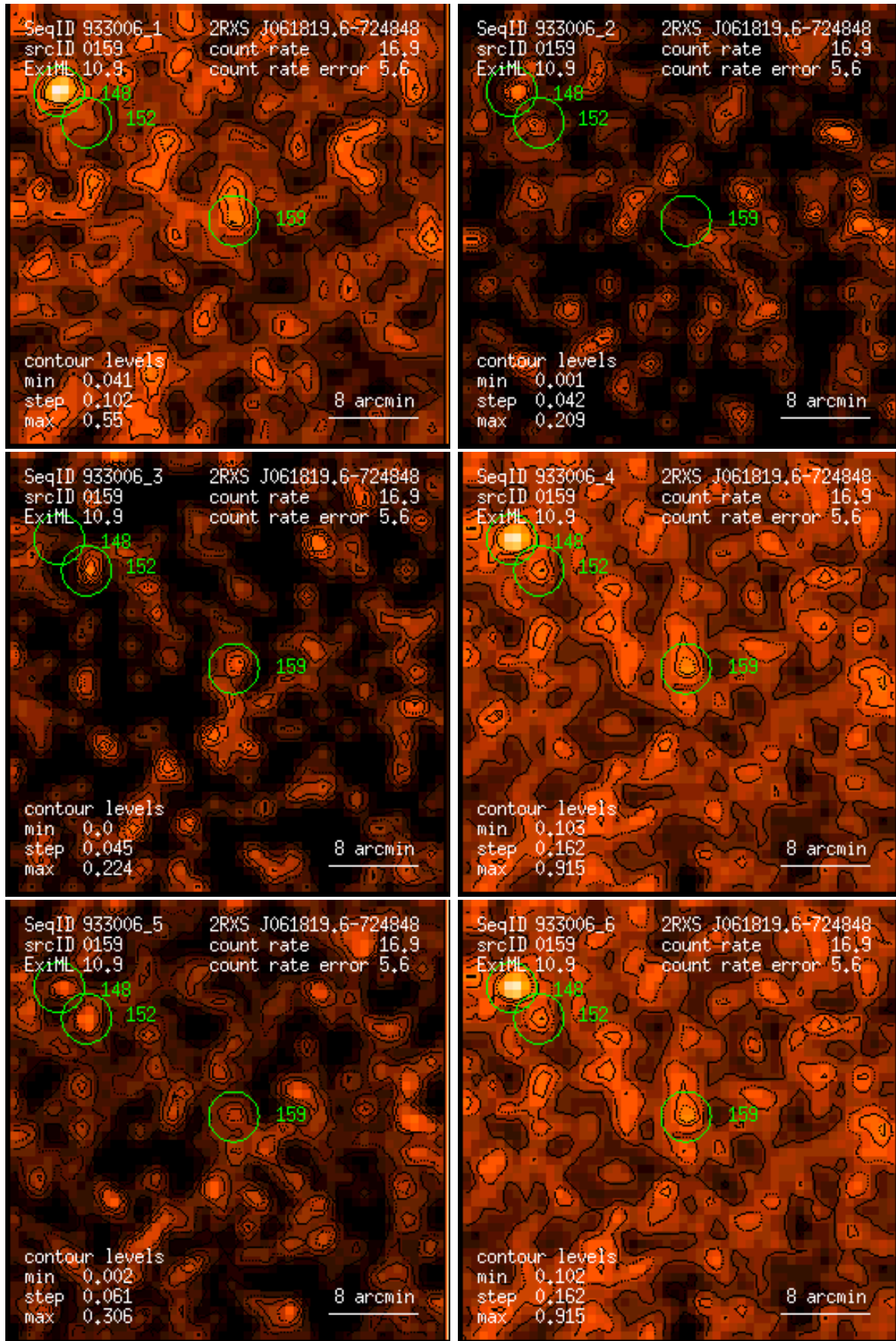
Figure 159: RASS 933006: detection 0159: band rate images, Gaussian filter: (1) PSPC channels 11 – 41, (2) 52 – 90, (3) 91 – 201, (4) 11 – 235, (5) 52 – 201, (6) 11 – 201. Broad band rates in counts/ks. Band rate contour levels in counts/ks/arcmin 2 .
