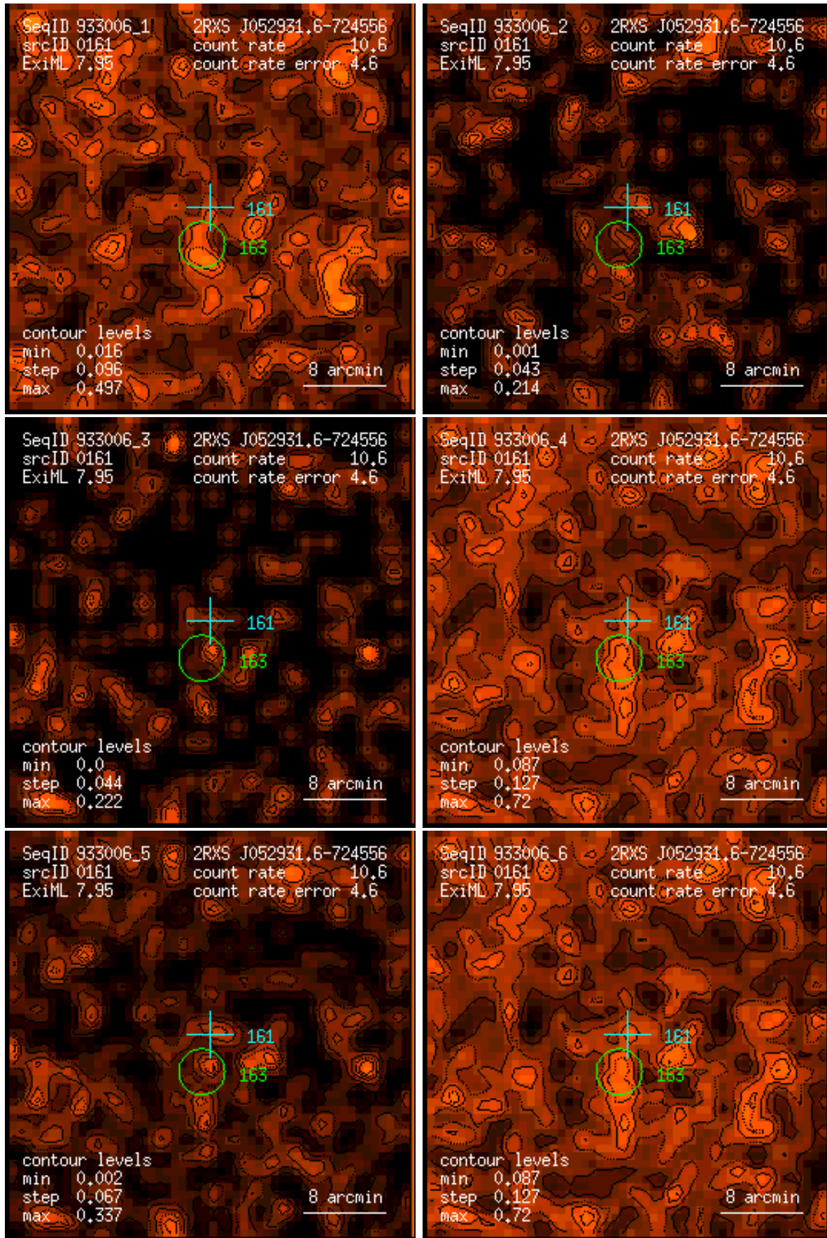
Figure 161: RASS 933006: detection 0161: band rate images, Gaussian filter: (1) PSPC channels 11 – 41, (2) 52 – 90, (3) 91 – 201, (4) 11 – 235, (5) 52 – 201, (6) 11 – 201. Broad band rates in counts/ks. Band rate contour levels in counts/ks/arcmin 2 .
