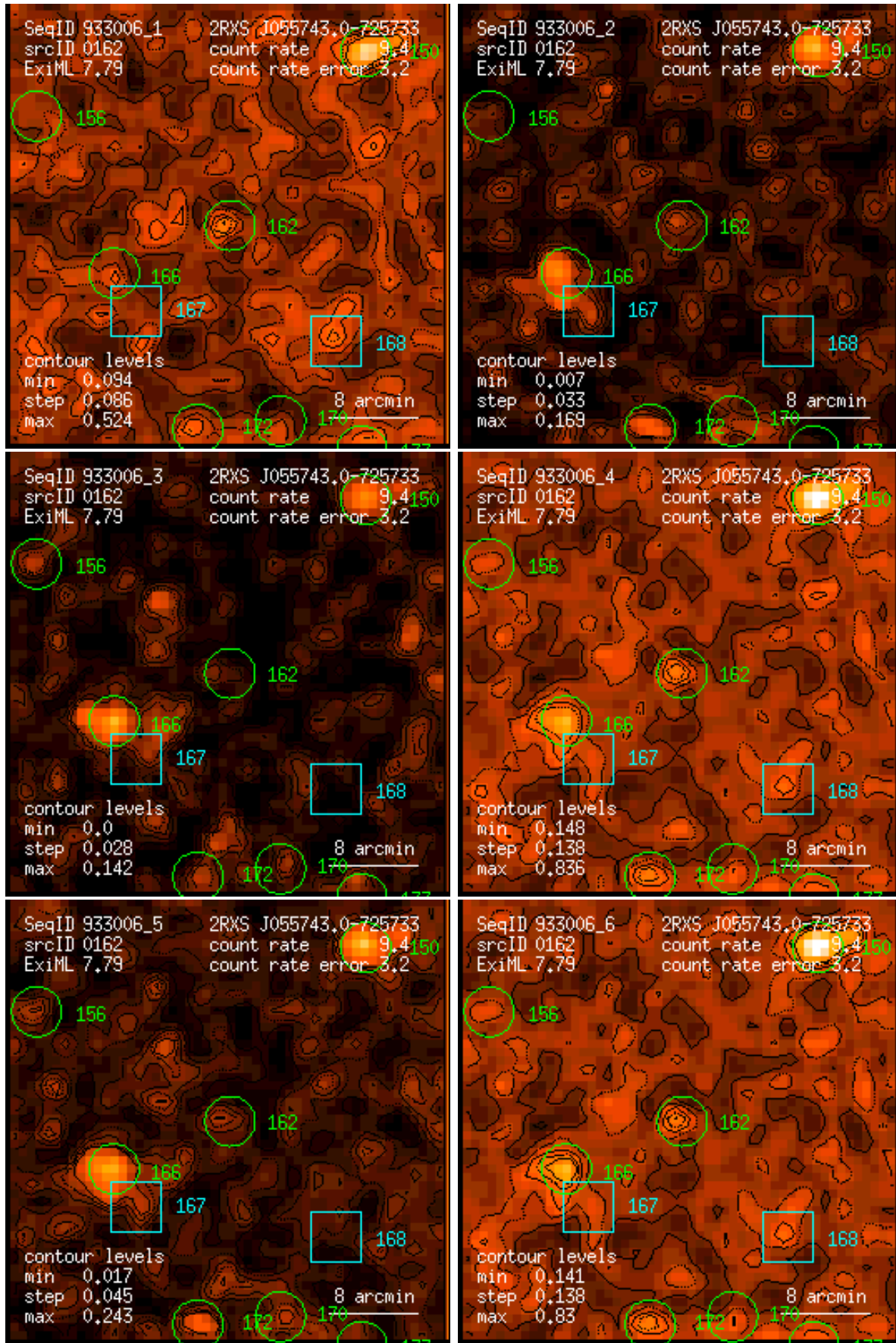
Figure 162: RASS 933006: detection 0162: band rate images, Gaussian filter: (1) PSPC channels 11 – 41, (2) 52 – 90, (3) 91 – 201, (4) 11 – 235, (5) 52 – 201, (6) 11 – 201. Broad band rates in counts/ks. Band rate contour levels in counts/ks/arcmin 2 .
