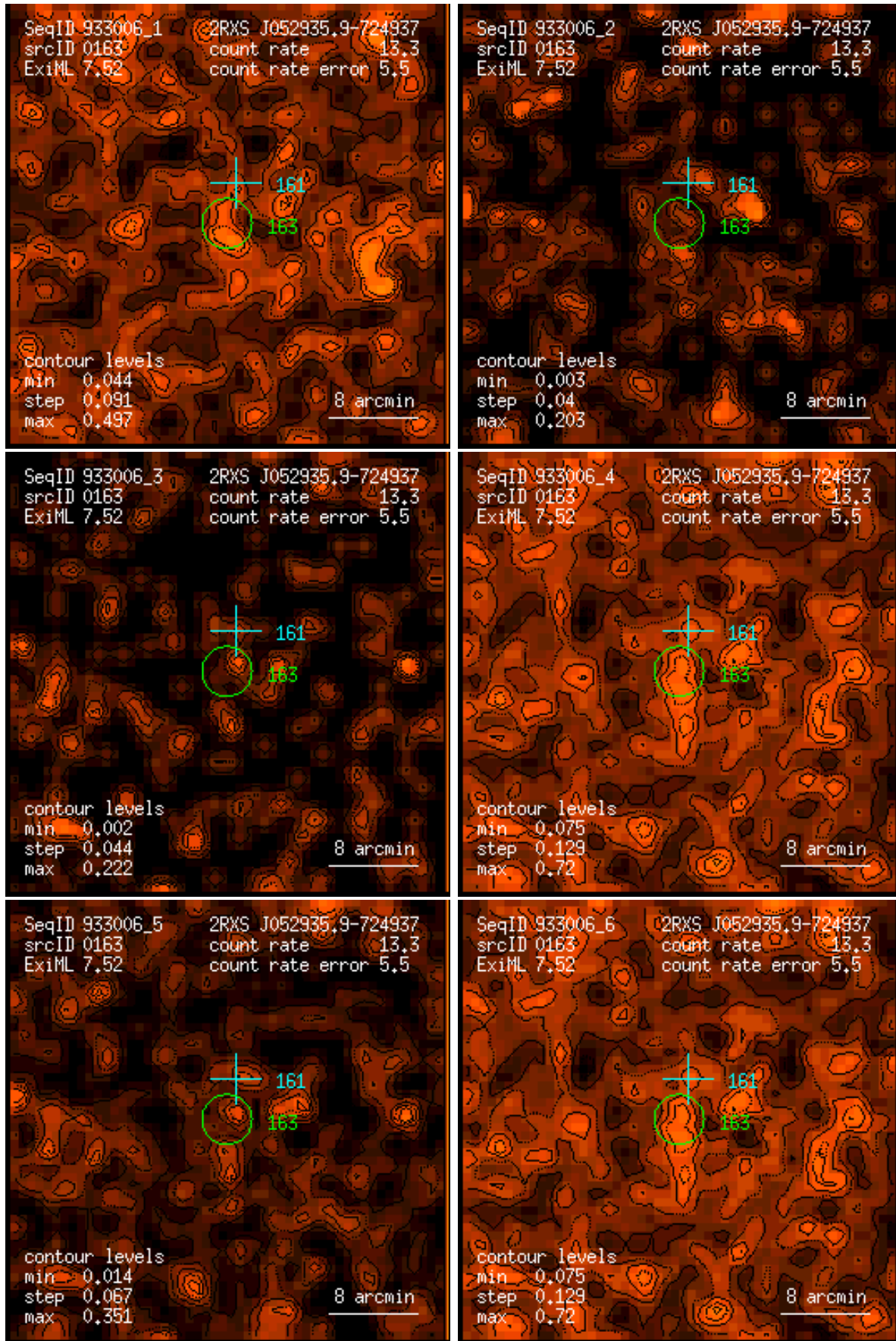
Figure 163: RASS 933006: detection 0163: band rate images, Gaussian filter: (1) PSPC channels 11 – 41, (2) 52 – 90, (3) 91 – 201, (4) 11 – 235, (5) 52 – 201, (6) 11 – 201. Broad band rates in counts/ks. Band rate contour levels in counts/ks/arcmin 2 .
