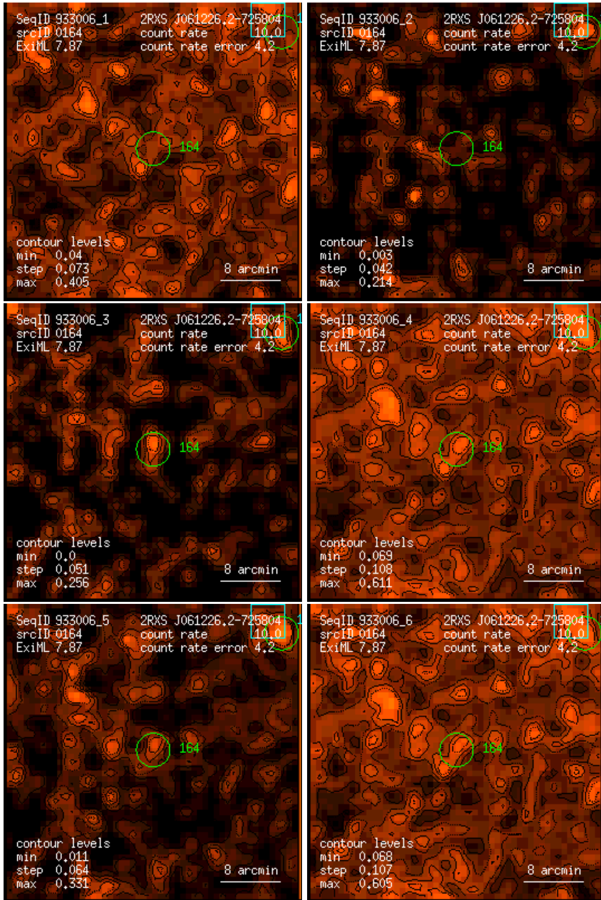
Figure 164: RASS 933006: detection 0164: band rate images, Gaussian filter: (1) PSPC channels 11 – 41, (2) 52 – 90, (3) 91 – 201, (4) 11 – 235, (5) 52 – 201, (6) 11 – 201. Broad band rates in counts/ks. Band rate contour levels in counts/ks/arcmin 2 .
