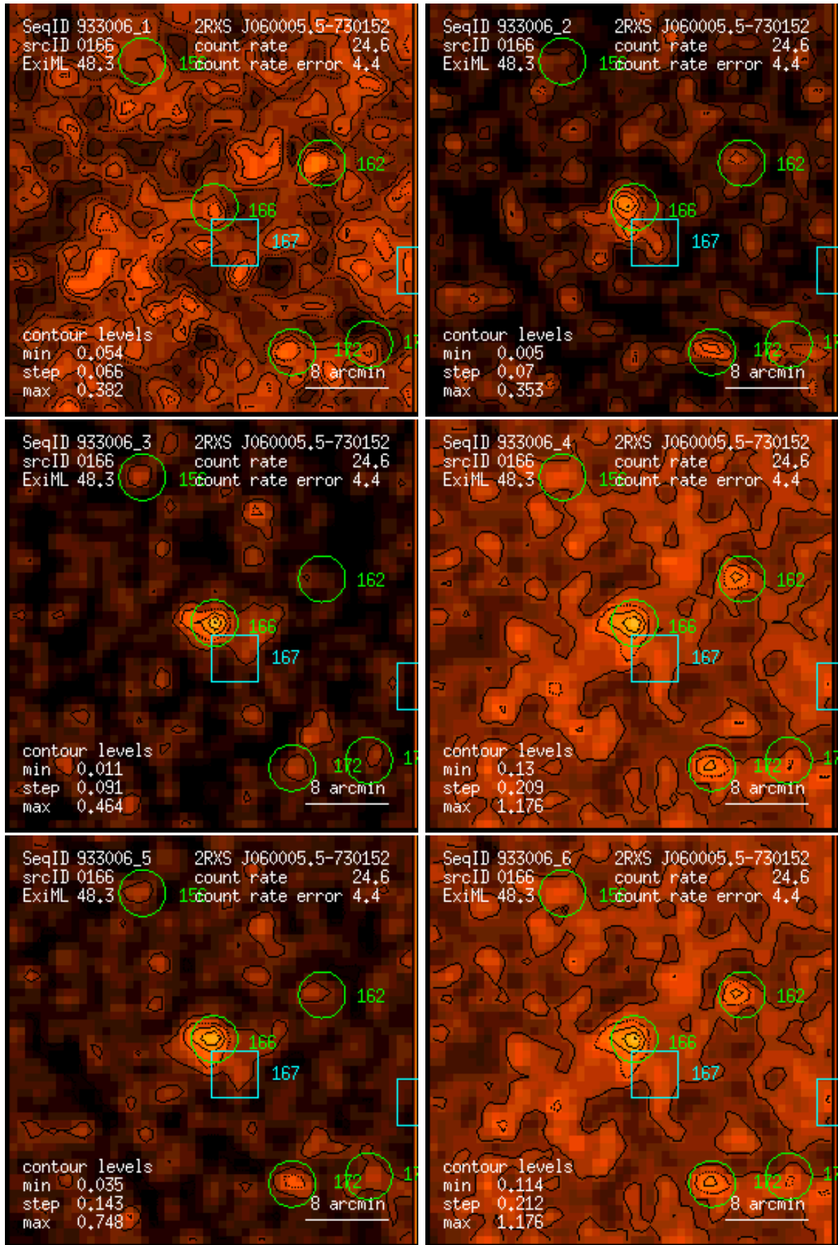
Figure 166: RASS 933006: detection 0166: band rate images, Gaussian filter: (1) PSPC channels 11 – 41, (2) 52 – 90, (3) 91 – 201, (4) 11 – 235, (5) 52 – 201, (6) 11 – 201. Broad band rates in counts/ks. Band rate contour levels in counts/ks/arcmin 2 .
