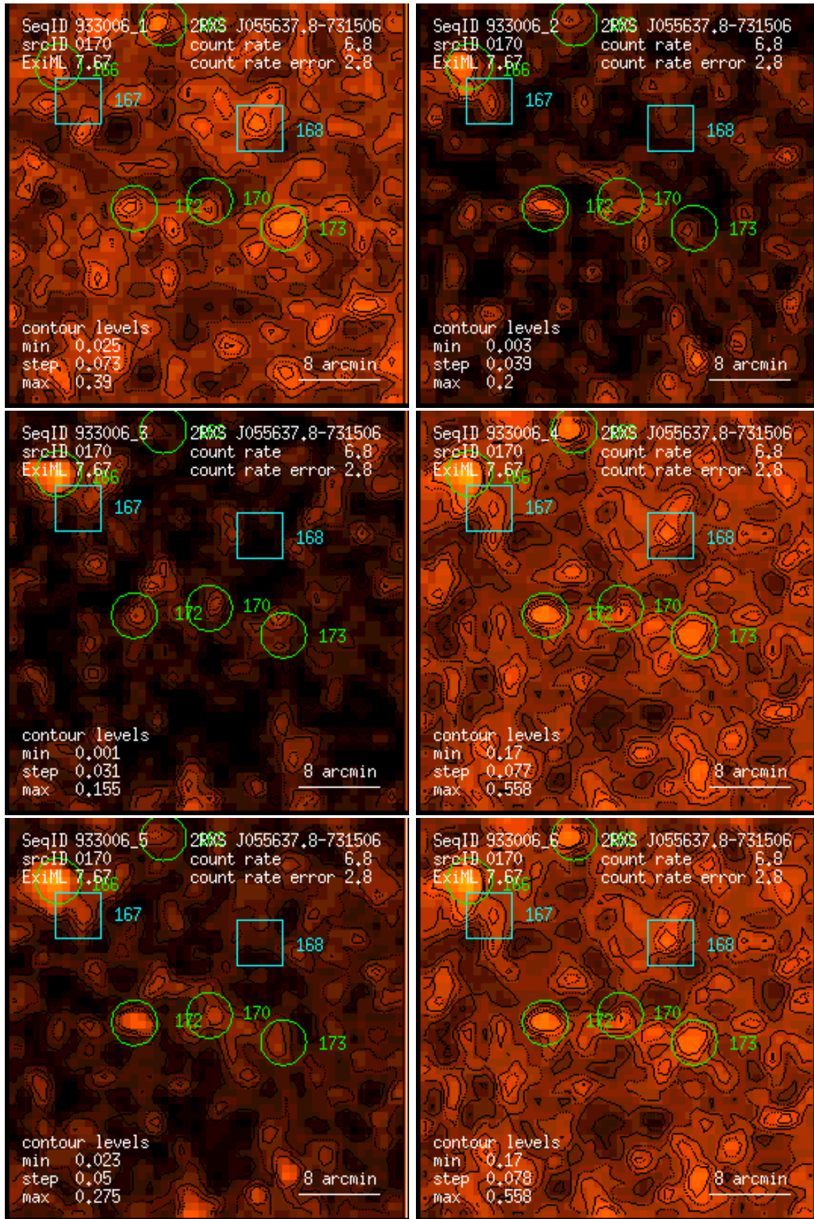
Figure 170: RASS 933006: detection 0170: band rate images, Gaussian filter: (1) PSPC channels 11 – 41, (2) 52 – 90, (3) 91 – 201, (4) 11 – 235, (5) 52 – 201, (6) 11 – 201. Broad band rates in counts/ks. Band rate contour levels in counts/ks/arcmin 2 .
