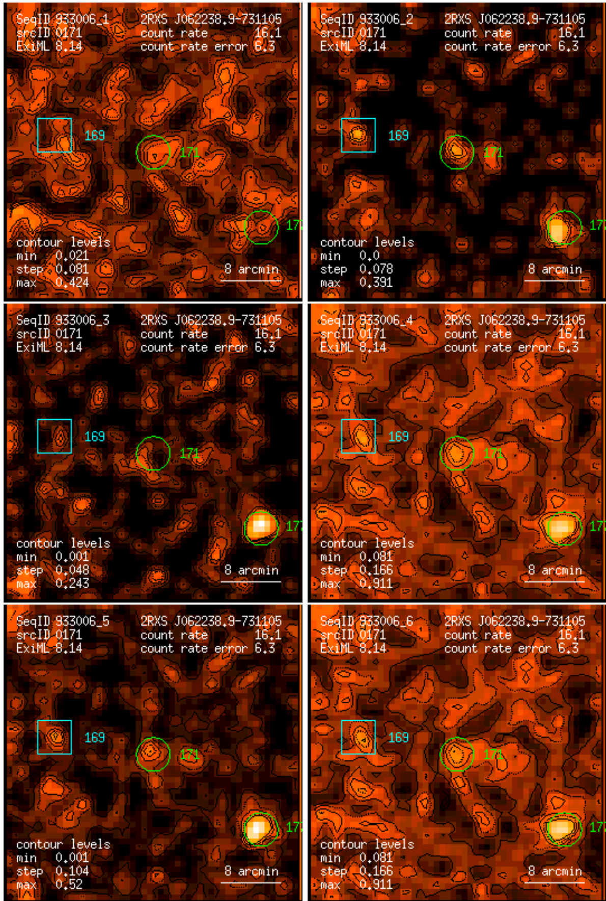
Figure 171: RASS 933006: detection 0171: band rate images, Gaussian filter: (1) PSPC channels 11 – 41, (2) 52 – 90, (3) 91 – 201, (4) 11 – 235, (5) 52 – 201, (6) 11 – 201. Broad band rates in counts/ks. Band rate contour levels in counts/ks/arcmin 2 .
