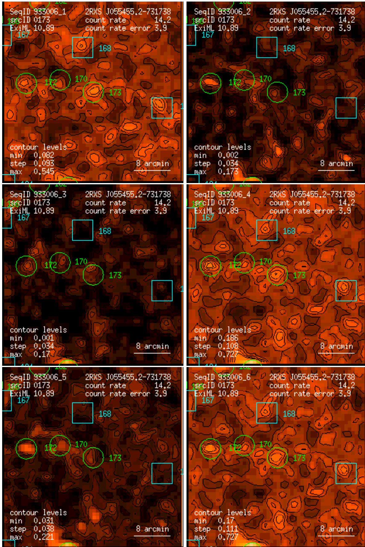
Figure 173: RASS 933006: detection 0173: band rate images, Gaussian filter: (1) PSPC channels 11 – 41, (2) 52 – 90, (3) 91 – 201, (4) 11 – 235, (5) 52 – 201, (6) 11 – 201. Broad band rates in counts/ks. Band rate contour levels in counts/ks/arcmin 2 .
