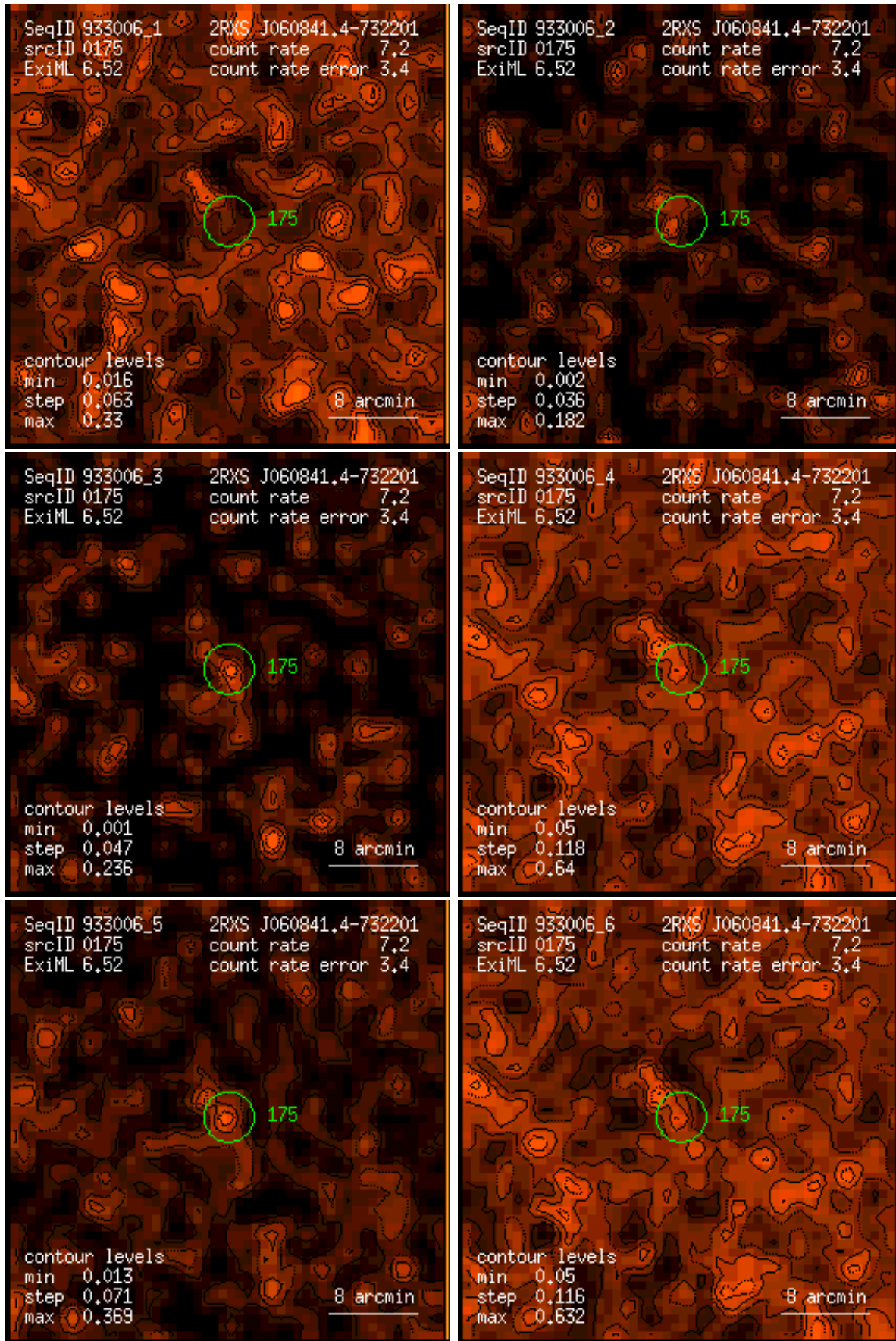
Figure 175: RASS 933006: detection 0175: band rate images, Gaussian filter: (1) PSPC channels 11 – 41, (2) 52 – 90, (3) 91 – 201, (4) 11 – 235, (5) 52 – 201, (6) 11 – 201. Broad band rates in counts/ks. Band rate contour levels in counts/ks/arcmin 2 .
