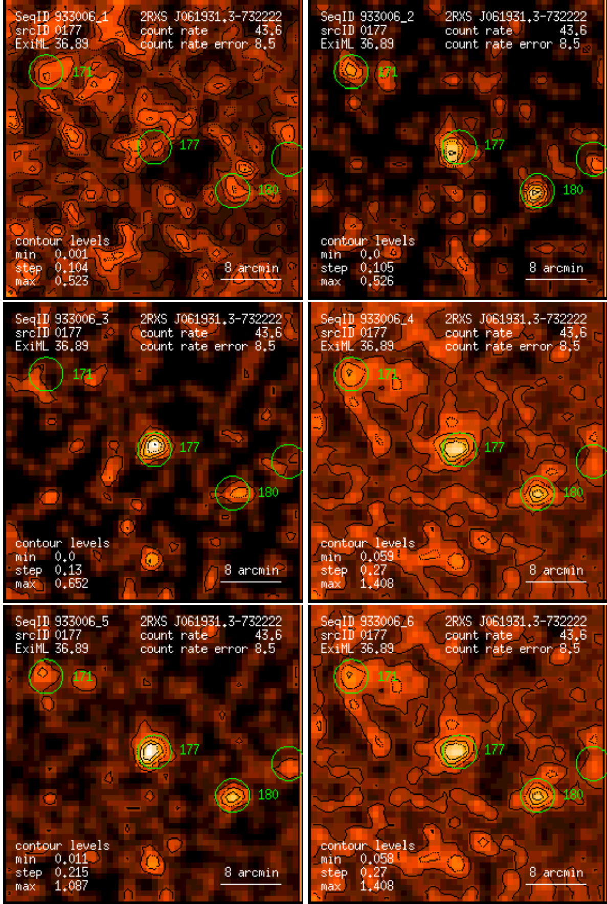
Figure 177: RASS 933006: detection 0177: band rate images, Gaussian filter: (1) PSPC channels 11 – 41, (2) 52 – 90, (3) 91 – 201, (4) 11 – 235, (5) 52 – 201, (6) 11 – 201. Broad band rates in counts/ks. Band rate contour levels in counts/ks/arcmin 2 .
