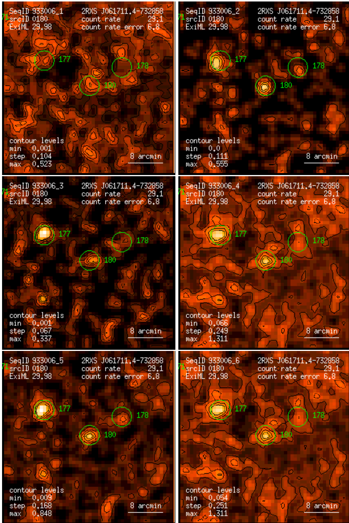
Figure 180: RASS 933006: detection 0180: band rate images, Gaussian filter: (1) PSPC channels 11 – 41, (2) 52 – 90, (3) 91 – 201, (4) 11 – 235, (5) 52 – 201, (6) 11 – 201. Broad band rates in counts/ks. Band rate contour levels in counts/ks/arcmin 2 .
