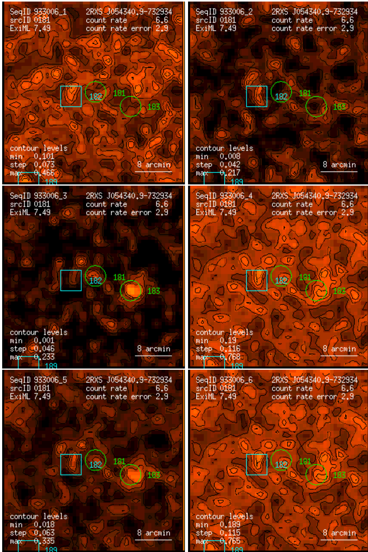
Figure 181: RASS 933006: detection 0181: band rate images, Gaussian filter: (1) PSPC channels 11 – 41, (2) 52 – 90, (3) 91 – 201, (4) 11 – 235, (5) 52 – 201, (6) 11 – 201. Broad band rates in counts/ks. Band rate contour levels in counts/ks/arcmin 2 .
