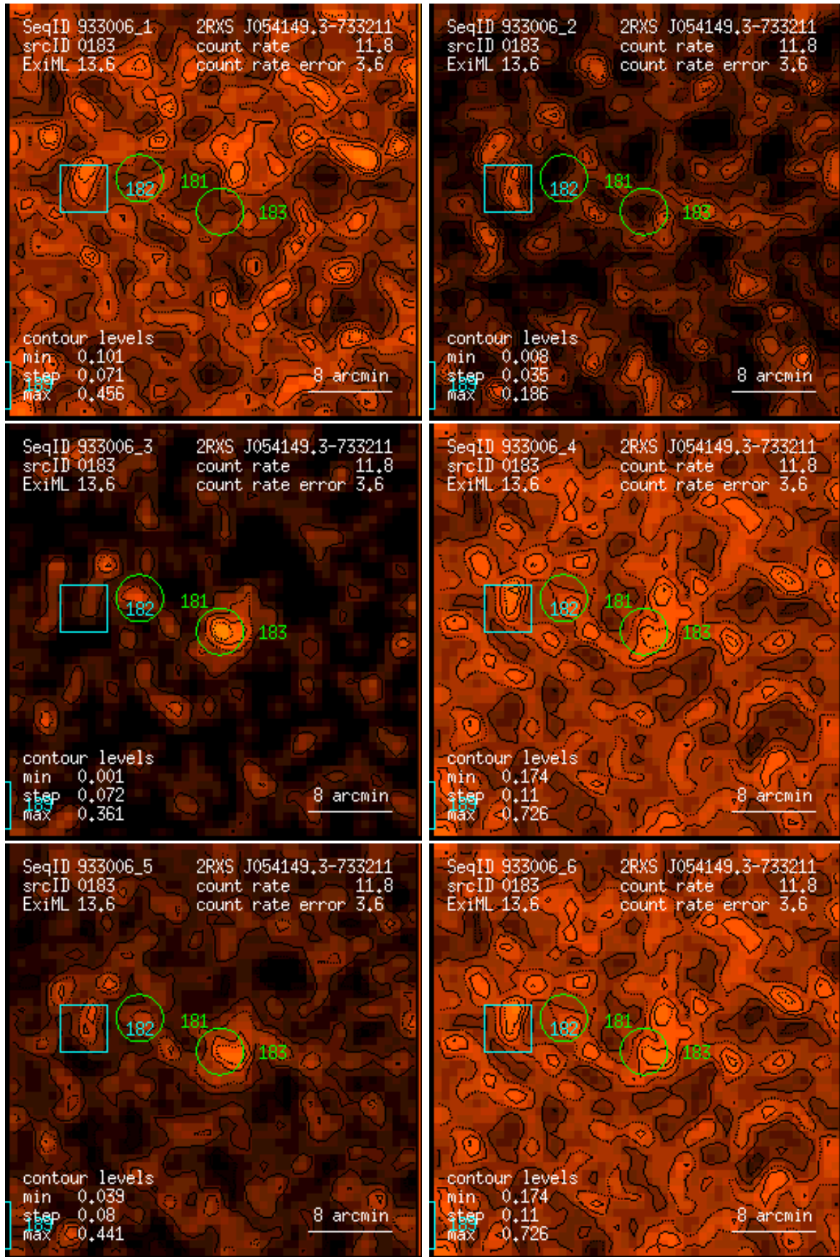
Figure 183: RASS 933006: detection 0183: band rate images, Gaussian filter: (1) PSPC channels 11 – 41, (2) 52 – 90, (3) 91 – 201, (4) 11 – 235, (5) 52 – 201, (6) 11 – 201. Broad band rates in counts/ks. Band rate contour levels in counts/ks/arcmin 2 .
