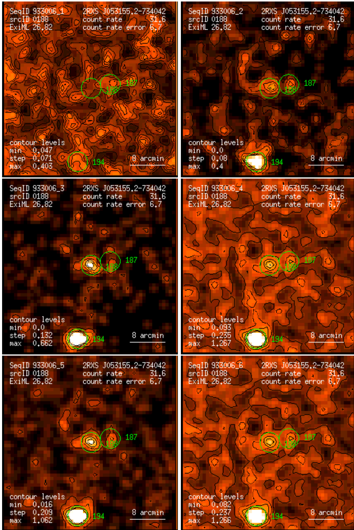
Figure 188: RASS 933006: detection 0188: band rate images, Gaussian filter: (1) PSPC channels 11 – 41, (2) 52 – 90, (3) 91 – 201, (4) 11 – 235, (5) 52 – 201, (6) 11 – 201. Broad band rates in counts/ks. Band rate contour levels in counts/ks/arcmin 2 .
